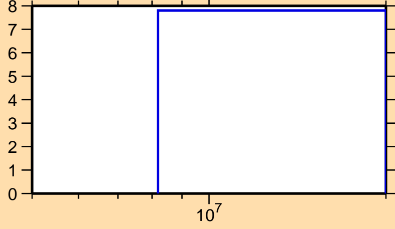
\Delta\sigma/\sigma vs. E for ^{41}\text{S}(n,el.)
