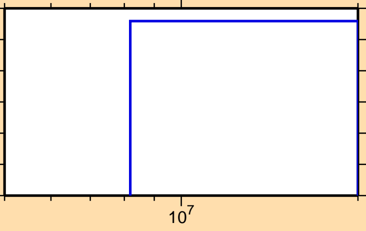
\sigma vs. E for ^{41}\text{S}(n,n\alpha)
