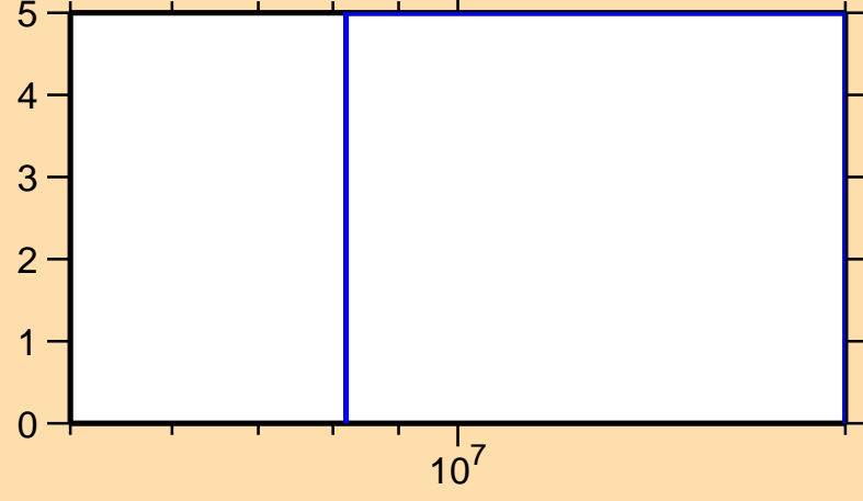
\Delta\sigma/\sigma vs. E for ^{41}\text{S}(n,\text{tot.})
