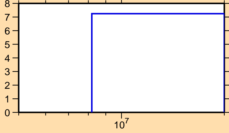
\Delta\sigma/\sigma vs. E for ^{42}\text{S}(n,\text{tot.})
