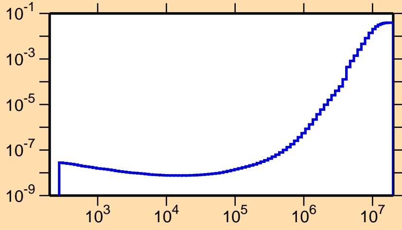
\sigma vs. E for ^{105}\text{Sb}(n,d)
