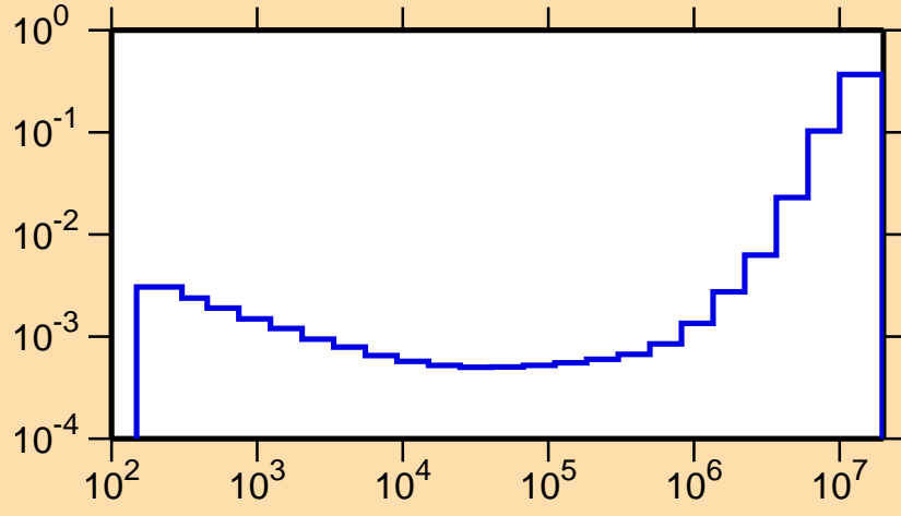
\sigma vs. E for ^{105}\text{Sb}(n,p\alpha)
