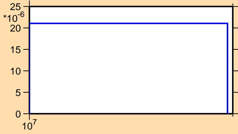
\sigma vs. E for ^{105}\text{Sb}(n,\text{pt})
