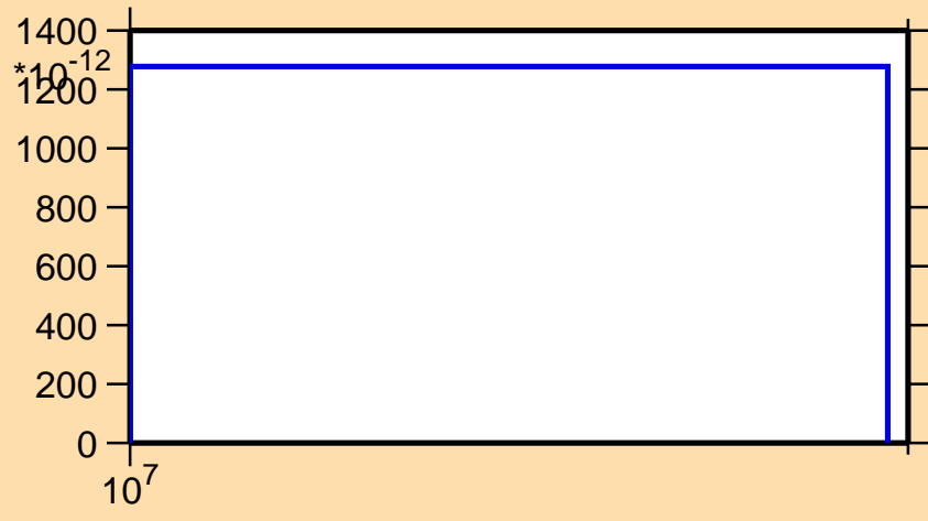
\sigma vs. E for ^{105}\text{Sb} (mt 34)
