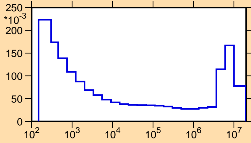
\sigma vs. E for ^{105}\text{Sb}(n,\alpha)
