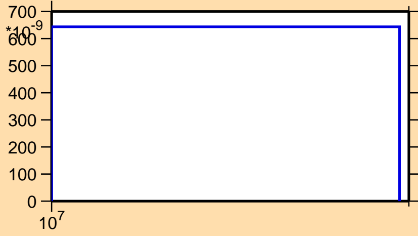
\sigma vs. E for ^{105}\text{Sb}(n,\text{nd})
