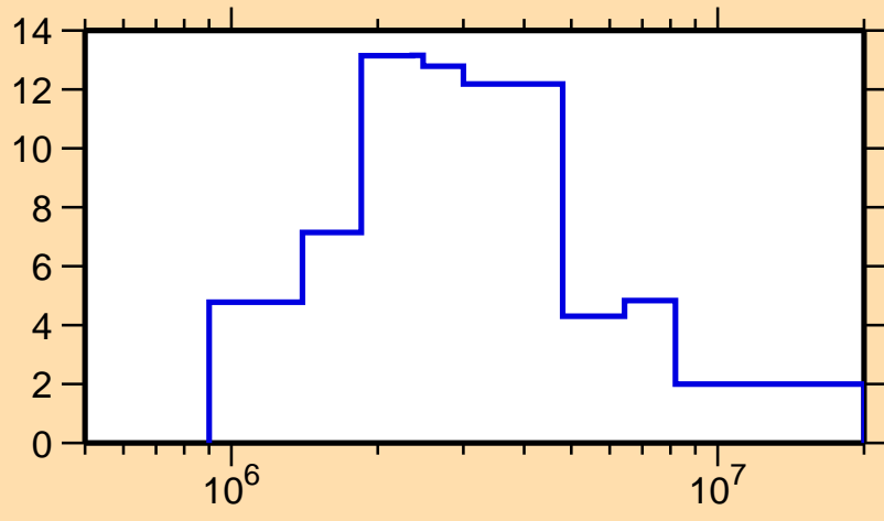
\Delta\sigma/\sigma vs. E for ^{105}\text{Sb}(n,\text{tot.})
