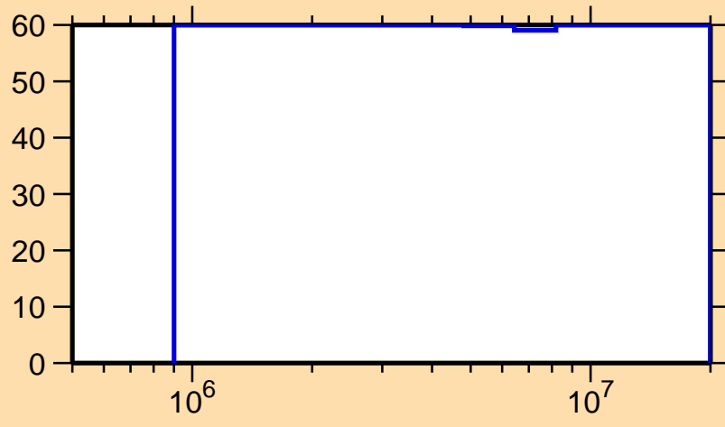
\Delta\sigma/\sigma vs. E for ^{105}\text{Sb}(n,n_1)
