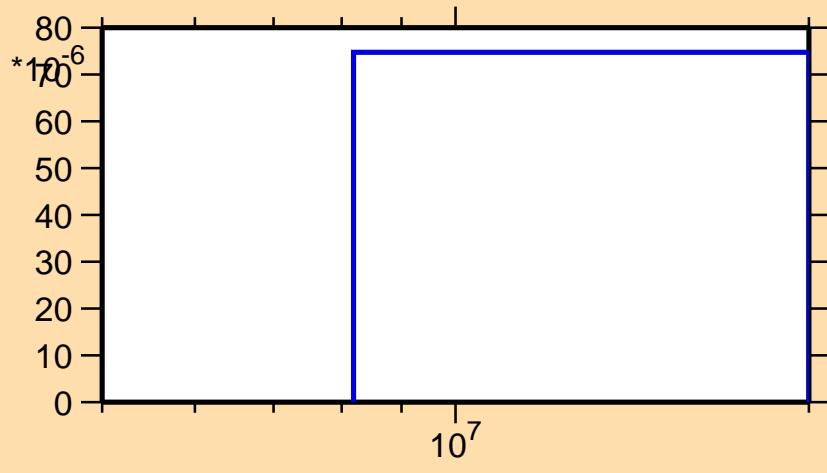
\sigma vs. E for ^{105}\text{Sb}(n,2n)
