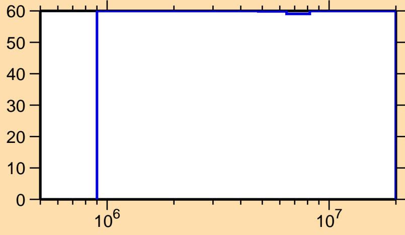
\Delta\sigma/\sigma vs. E for ^{105}\text{Sb}(n,n_1)
