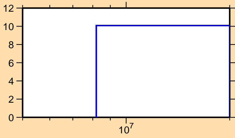
\Delta\sigma/\sigma vs. E for ^{105}\text{Sb}(n,\text{nonel.})
