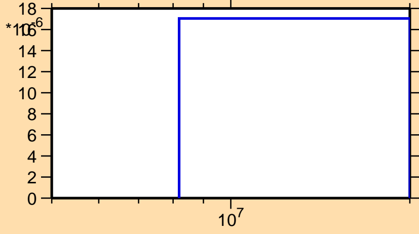
\sigma vs. E for ^{105}\text{Sb}(n,\text{pt})
