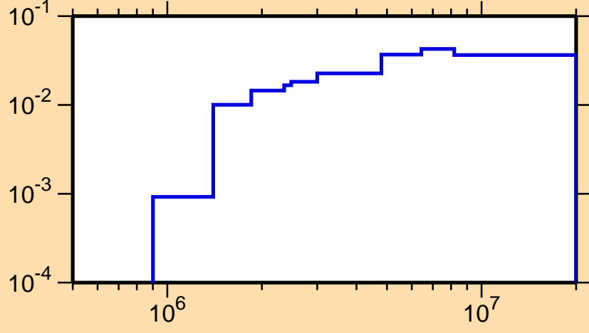
\sigma vs. E for ^{105}\text{Sb}(n,\text{inel.})
