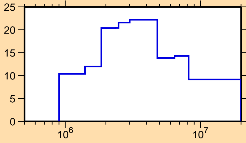
\Delta\sigma/\sigma vs. E for ^{105}\text{Sb}(n,\text{el.})
