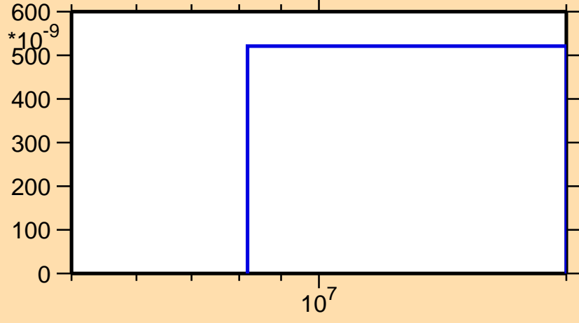
\sigma vs. E for ^{105}\text{Sb}(n,nd)
