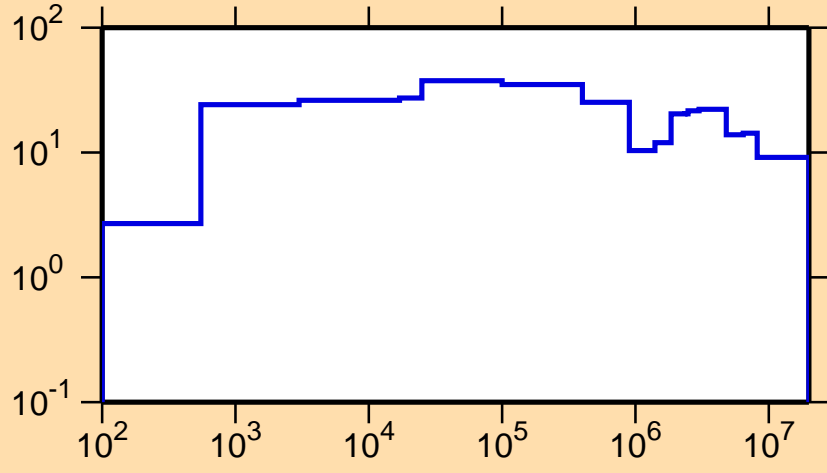
\Delta\sigma/\sigma vs. E for ^{105}\text{Sb}(n,\text{el.})
