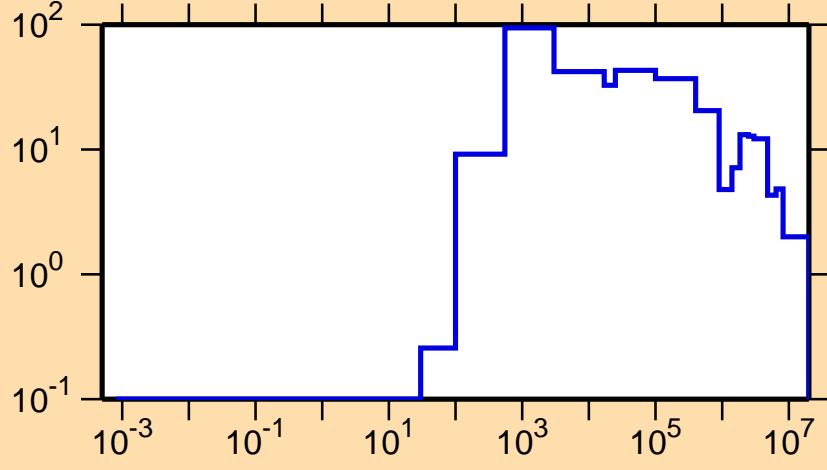
\Delta\sigma/\sigma vs. E for ^{105}\text{Sb}(n,\text{tot.})
