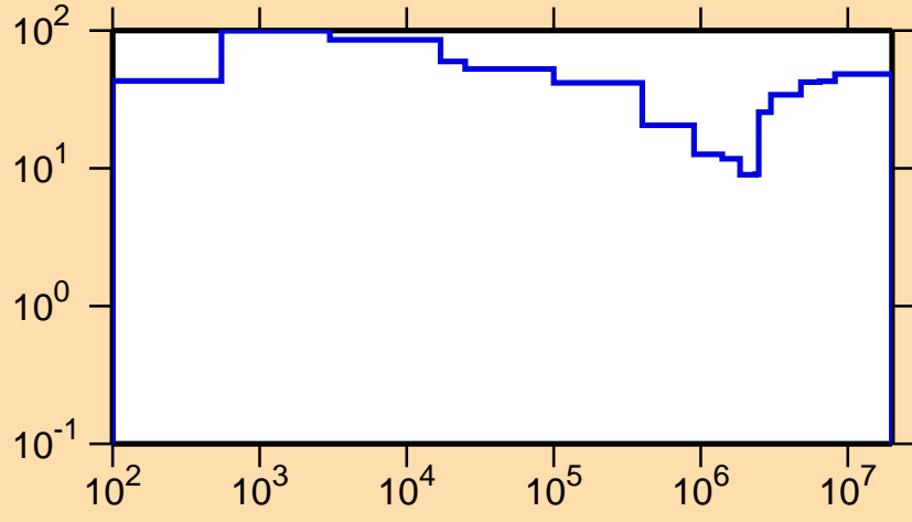
\Delta\sigma/\sigma vs. E for ^{105}\text{Sb}(n,p)
