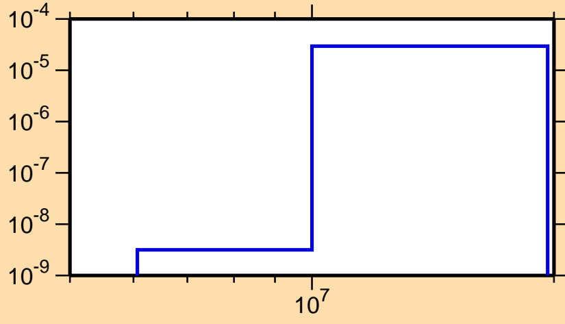
\sigma vs. E for ^{107}\text{Sb}(\text{mt117})
