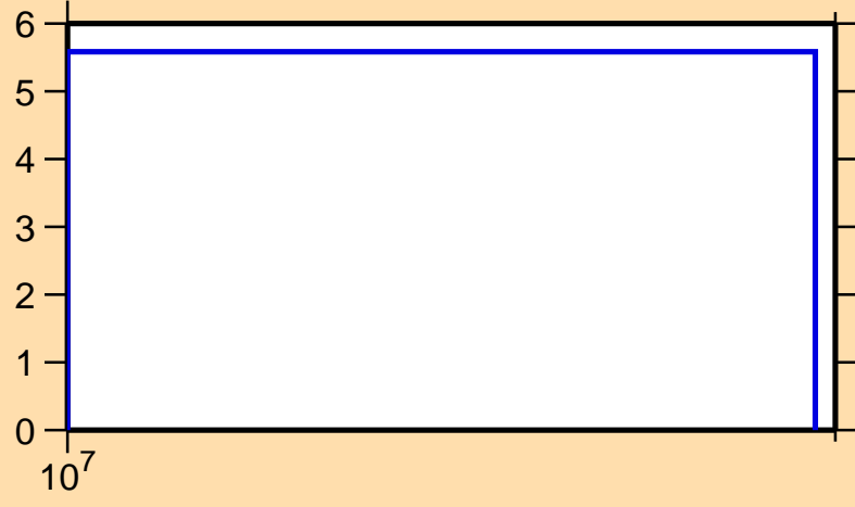
\Delta\sigma/\sigma vs. E for ^{107}\text{Sb}(n,\text{el.})
