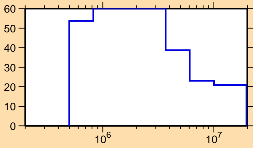
\Delta\sigma/\sigma vs. E for ^{107}\text{Sb}(n,n_1)
