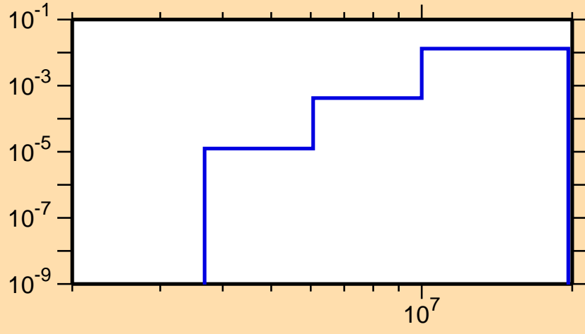
\sigma vs. E for ^{107}\text{Sb}(n,n\alpha)
