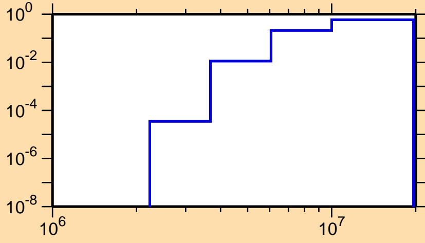
\sigma vs. E for ^{107}\text{Sb}(n,np)
