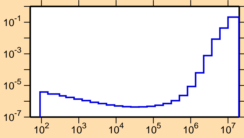
\sigma vs. E for ^{107}\text{Sb}(n,p\alpha)
