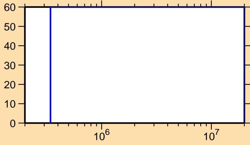
\Delta\sigma/\sigma vs. E for ^{108}\text{Sb}(n,n\text{cont.})
