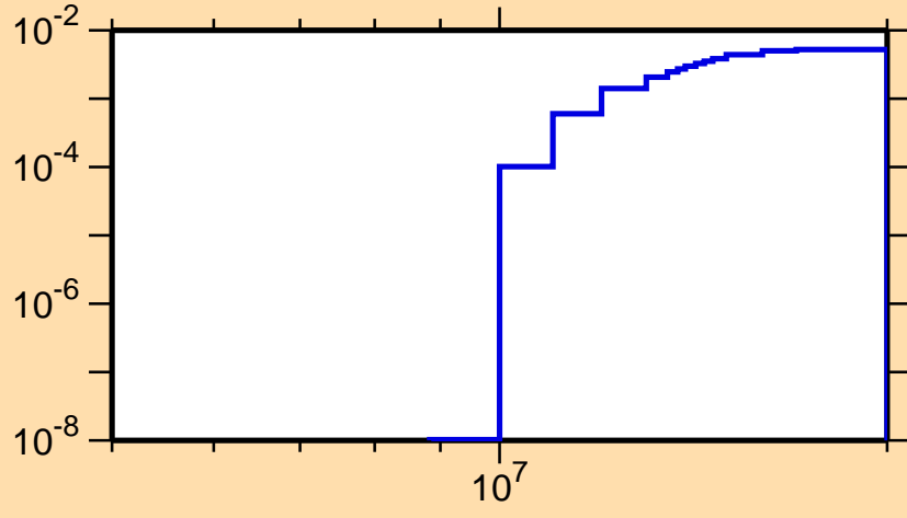
\sigma vs. E for ^{108}\text{Sb}(n,2n)
