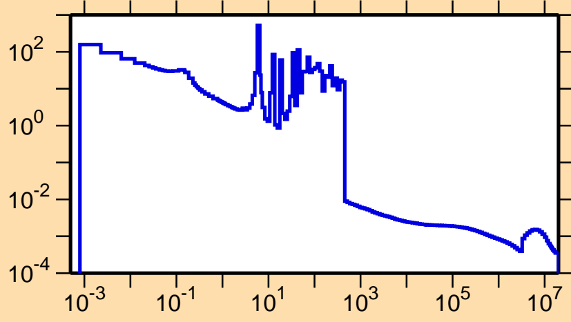
\sigma vs. E for ^{108}\text{Sb}(n,\gamma)
