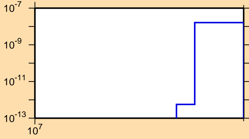
\sigma vs. E for ^{108}\text{Sb}(n,nt)
