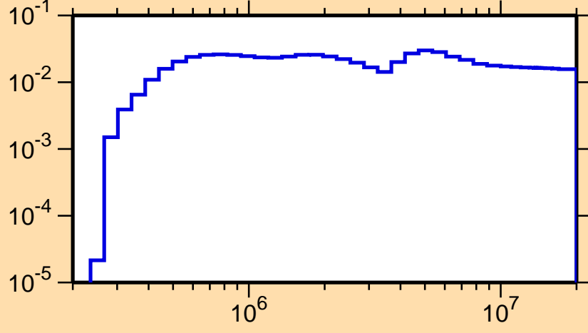
\sigma vs. E for ^{108}\text{Sb}(n,\text{inel.})
