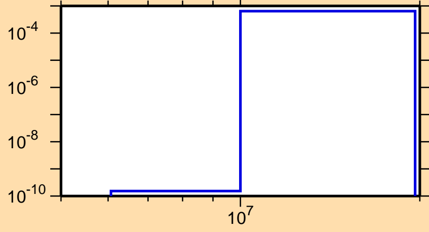
\sigma vs. E for ^{108}\text{Sb}(n,pd)
