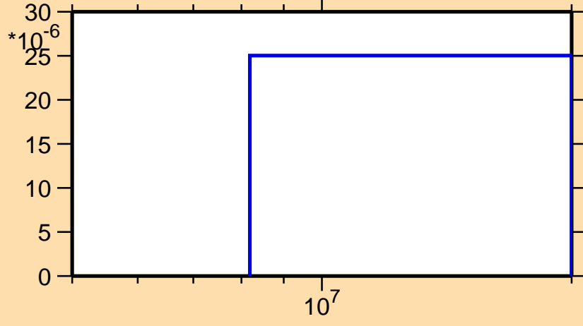
\sigma vs. E for ^{108}\text{Sb}(n,\text{nd})
