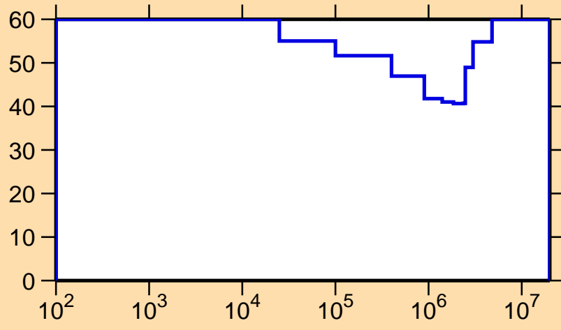
\Delta\sigma/\sigma vs. E for ^{108}\text{Sb}(n,p)
