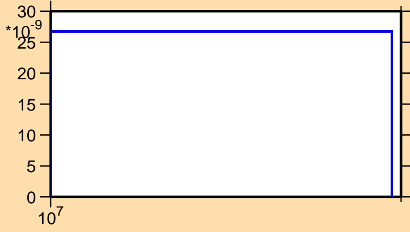
\sigma vs. E for ^{109}\text{Sb}(n,\text{pt})
