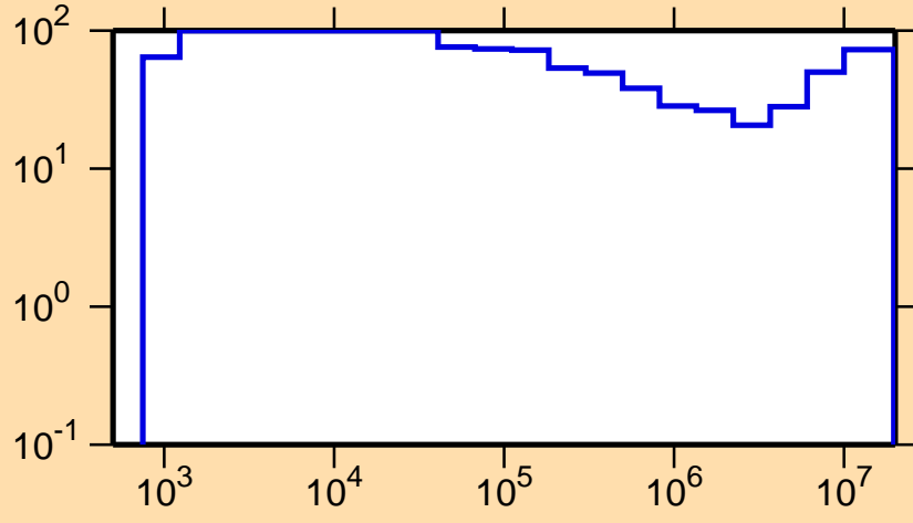
\Delta\sigma/\sigma vs. E for ^{109}\text{Sb}(n,p)
