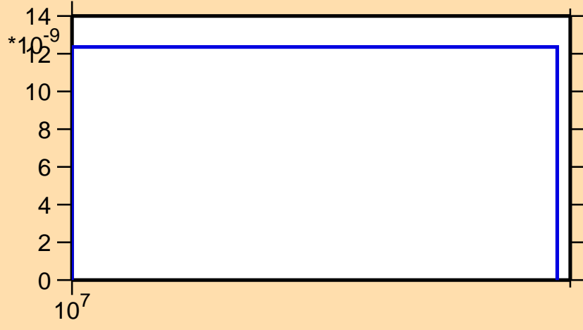
\sigma vs. E for ^{109}\text{Sb}(n,2n\alpha)
