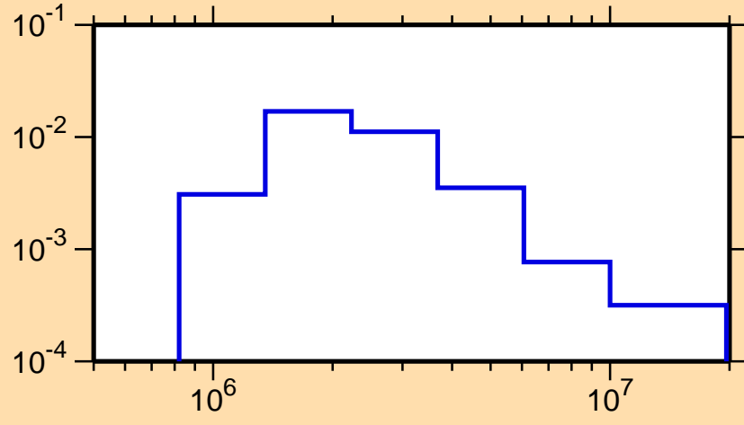
\sigma vs. E for ^{109}\text{Sb}(n,n_4)
