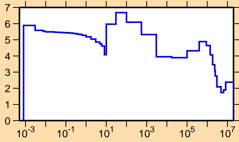
\sigma vs. E for ^{109}\text{Sb}(n,\text{el.})
