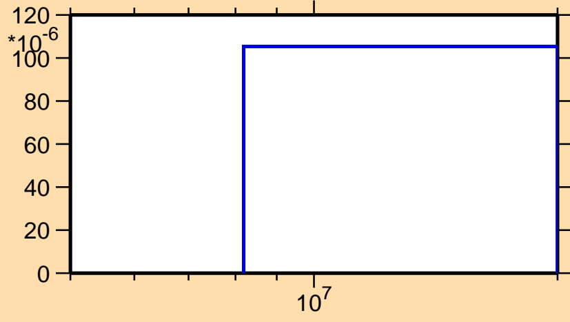
\sigma vs. E for ^{109}\text{Sb}(\text{mt } 45)
