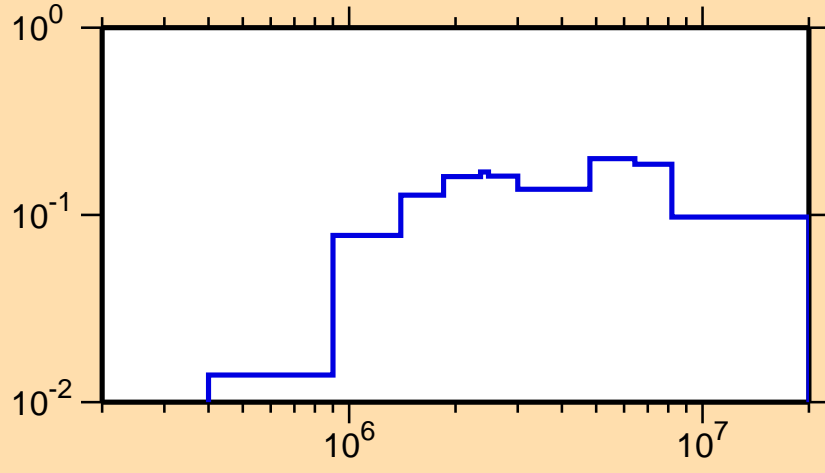
\sigma vs. E for ^{109}\text{Sb}(n,\text{inel.})
