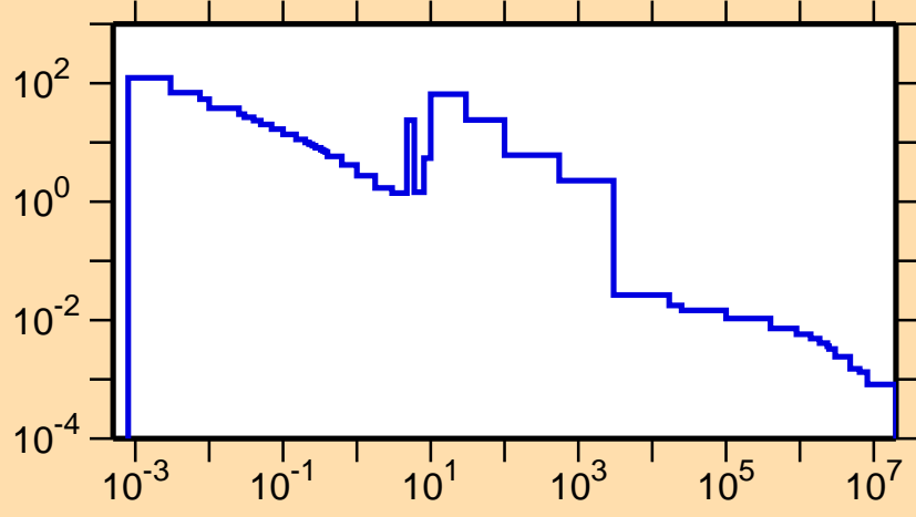
\sigma vs. E for ^{109}\text{Sb}(n,\gamma)
