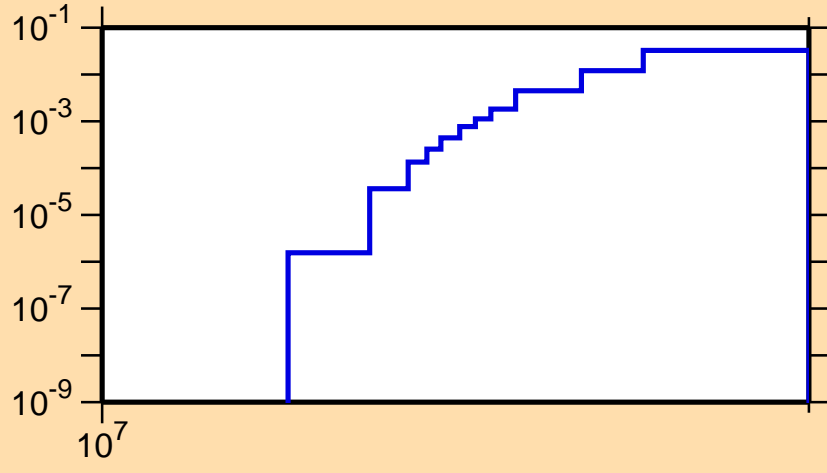
\sigma vs. E for ^{110}\text{Sb}(n,2np)
