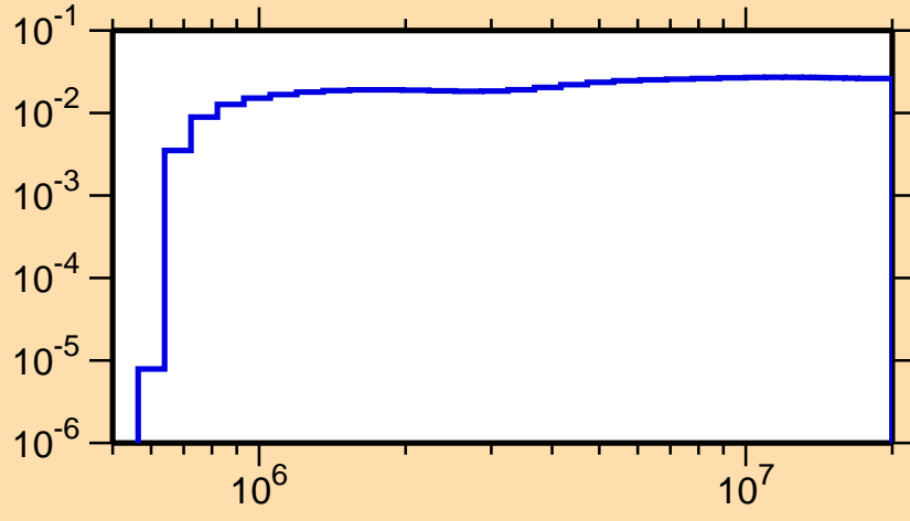
\sigma vs. E for ^{110}\text{Sb}(n,n_4)
