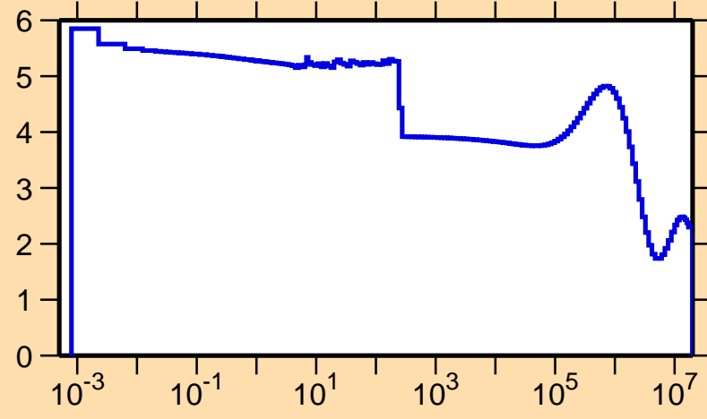
\sigma vs. E for ^{110}\text{Sb}(n,\text{el.})
