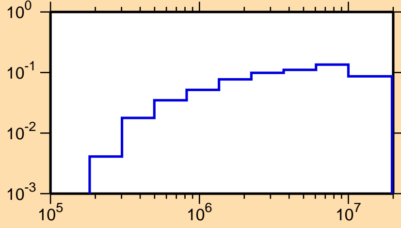
\sigma vs. E for ^{110}\text{Sb}(n,\text{inel.})
