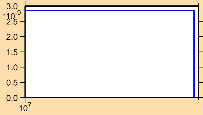
\sigma vs. E for ^{110}\text{Sb} (mt 34)
