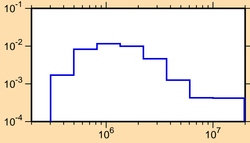
\sigma vs. E for ^{110}\text{Sb}(n,n_3)
