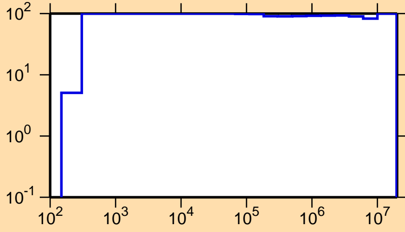
\Delta\sigma/\sigma vs. E for ^{110}\text{Sb}(n,\gamma)
