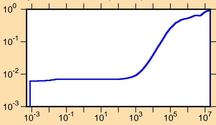
\mu vs. E for ^{111}\text{Sb}(\text{mt251})
