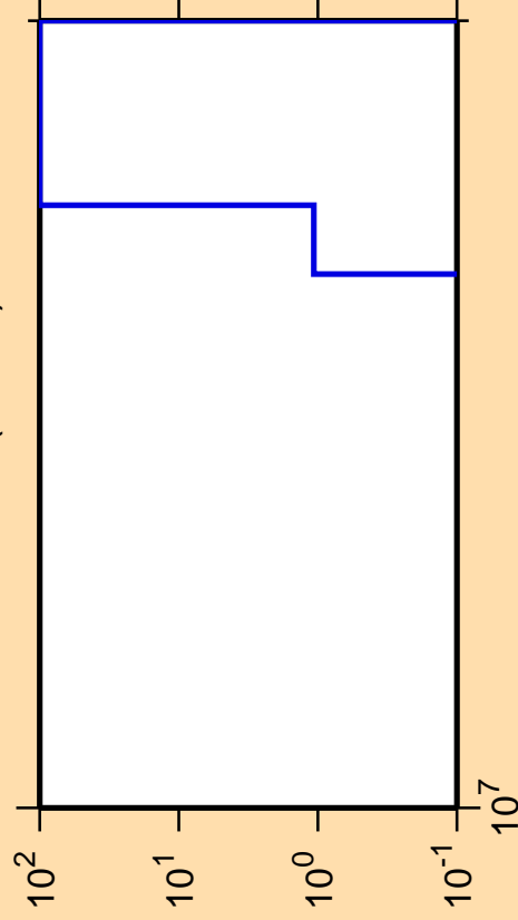
\Delta\sigma/\sigma vs. E for ^{111}\text{Sb} (mt 34)
