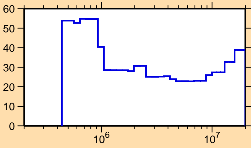
\Delta\sigma/\sigma vs. E for ^{111}\text{Sb}(n,n_1)
