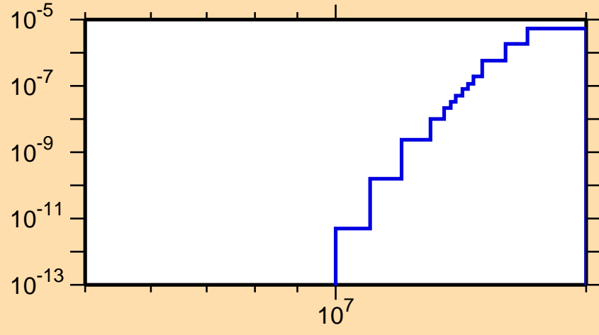
\sigma vs. E for ^{111}\text{Sb}(\text{mt117})
