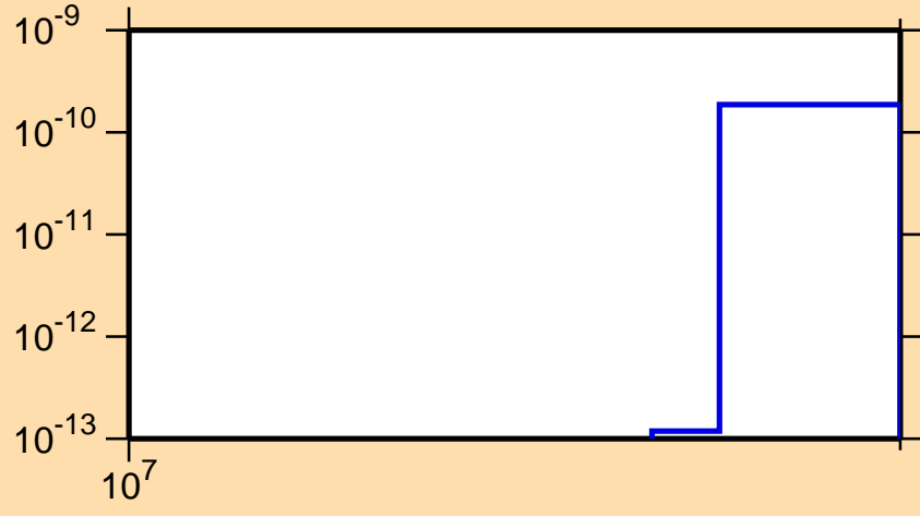
\sigma vs. E for ^{111}\text{Sb} (mt 34)
