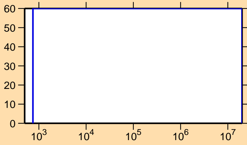
\Delta\sigma/\sigma vs. E for ^{111}\text{Sb}(n,\gamma)
