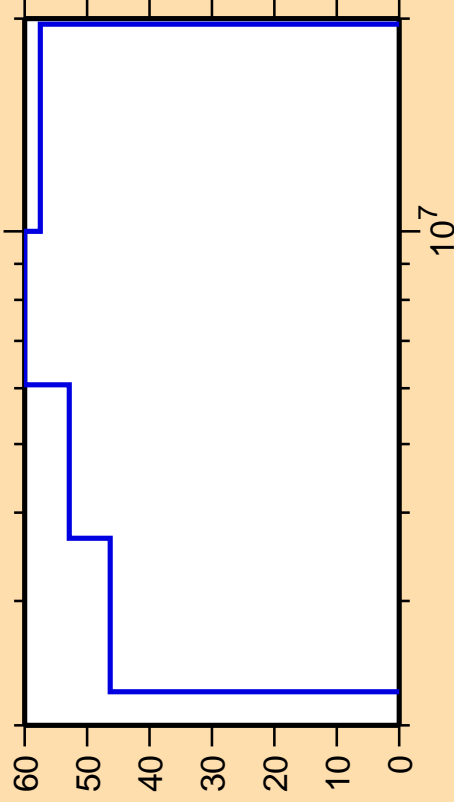
\Delta\sigma/\sigma vs. E for ^{111}\text{Sb}(n,n\text{cont.})
