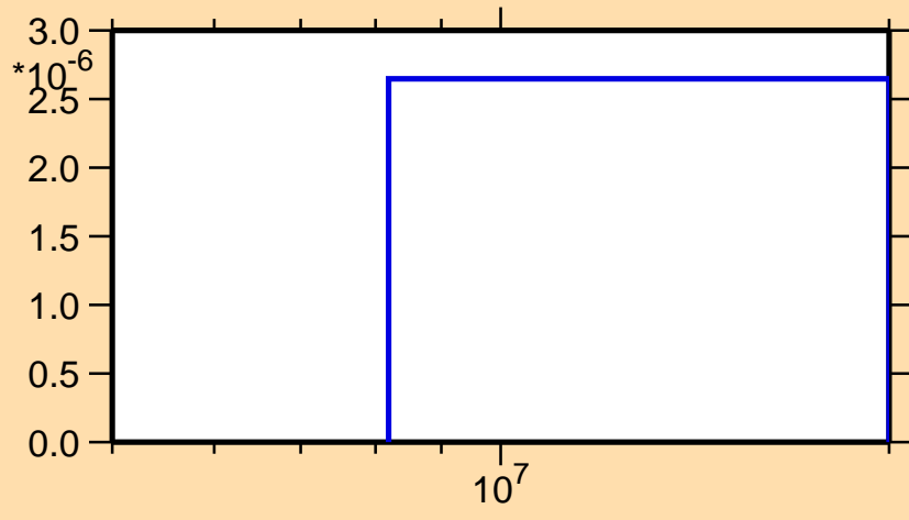
\sigma vs. E for ^{111}\text{Sb}(n,pd)
