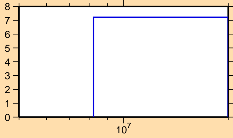
\Delta\sigma/\sigma vs. E for ^{111}\text{Sb}(n,\text{nonel.})
