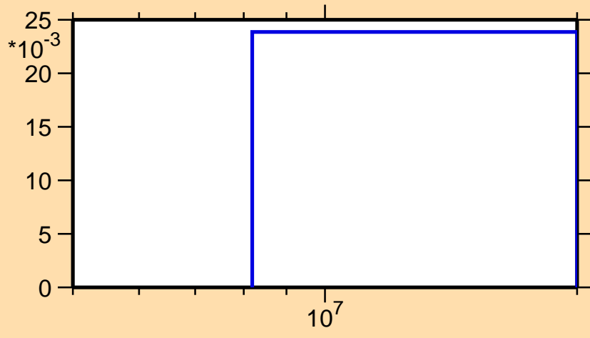
\sigma vs. E for ^{111}\text{Sb}(n,2n)
