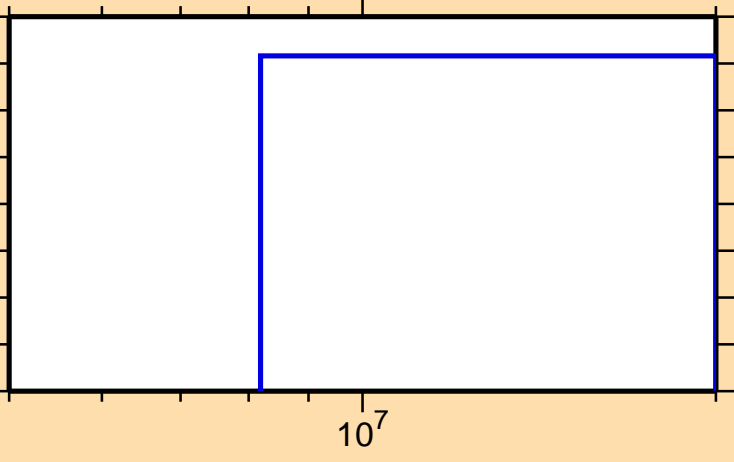
\sigma vs. E for ^{111}\text{Sb}(\text{mt } 45)
