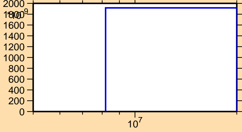
\sigma vs. E for ^{111}\text{Sb}(n,\text{nd})
