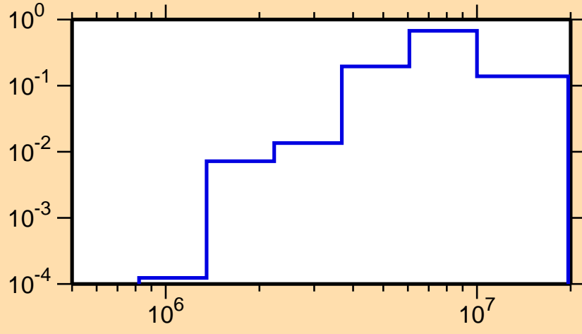
\sigma vs. E for ^{112}\text{Sb}(n,n\text{cont.})
