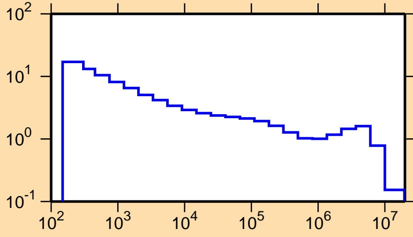
\sigma vs. E for ^{112}\text{Sb}(n,p)
