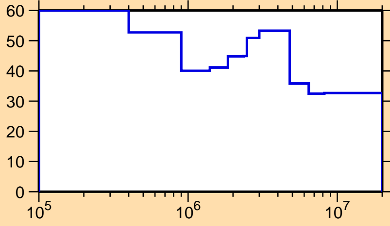
\Delta\sigma/\sigma vs. E for ^{112}\text{Sb}(n,n_1)
