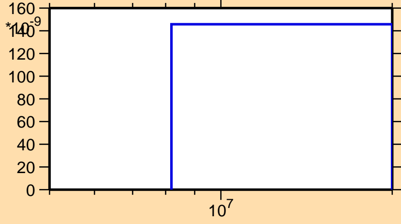
\sigma vs. E for ^{112}\text{Sb}(n,\text{pd})
