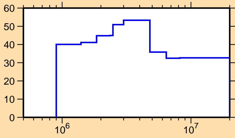
\Delta\sigma/\sigma vs. E for ^{112}\text{Sb}(n,n_1)
