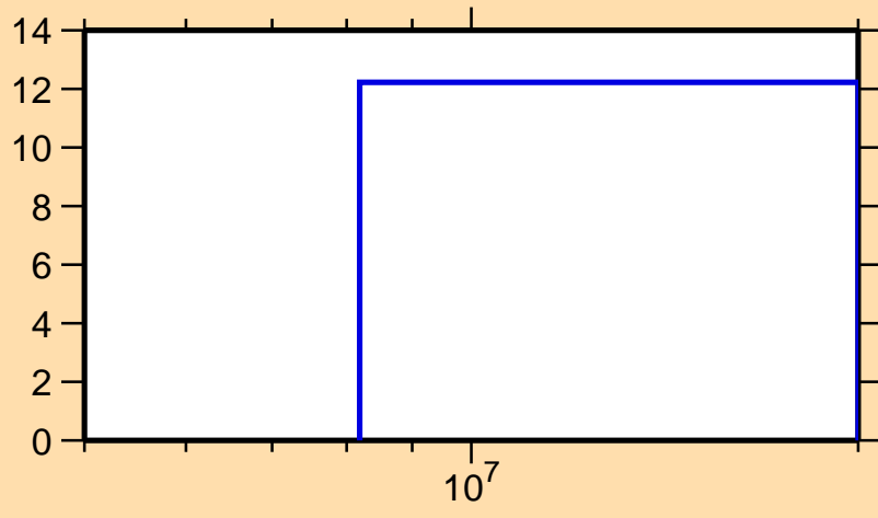
\Delta\sigma/\sigma vs. E for ^{112}\text{Sb}(n,\text{tot.})
