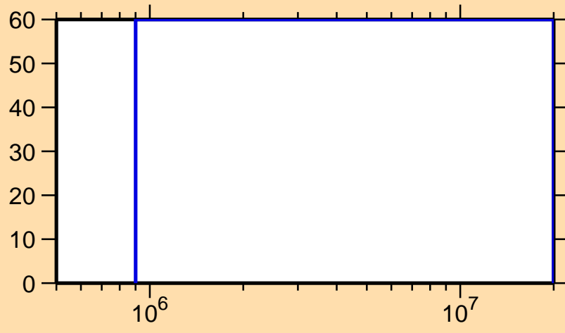
\Delta\sigma/\sigma vs. E for ^{112}\text{Sb}(n,n\text{cont.})
