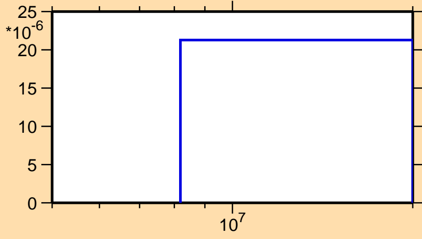
\sigma vs. E for ^{112}\text{Sb}(n,nd)
