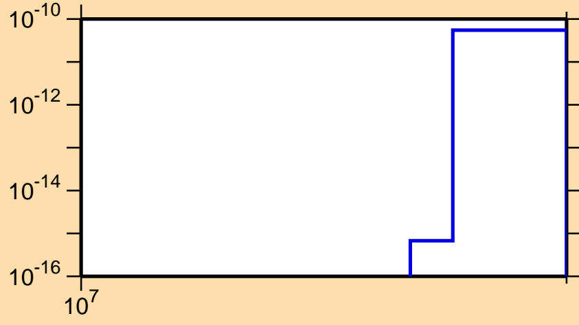
\sigma vs. E for ^{113}\text{Sb}(n,\text{pt})
