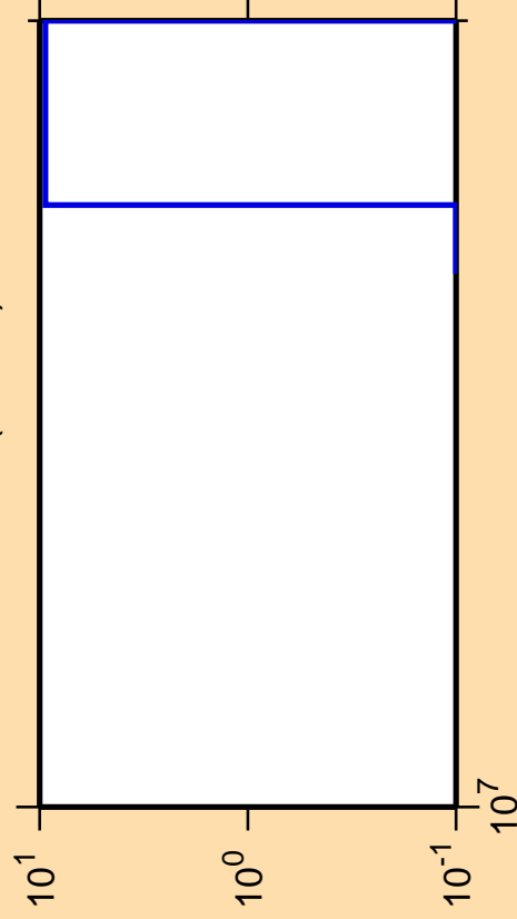
\Delta\sigma/\sigma vs. E for ^{113}\text{Sb} (mt 34)
