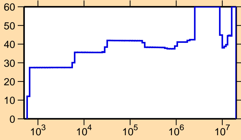
\Delta\sigma/\sigma vs. E for ^{113}\text{Sb}(n,\gamma)
