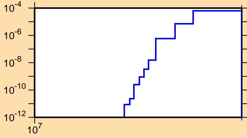
\sigma vs. E for ^{113}\text{Sb}(n,\text{nd})
