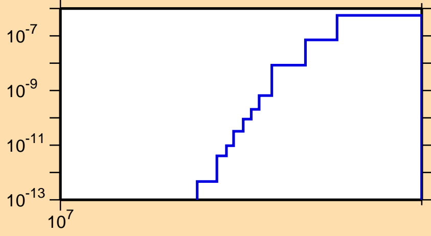
\sigma vs. E for ^{113}\text{Sb}(n,pd)
