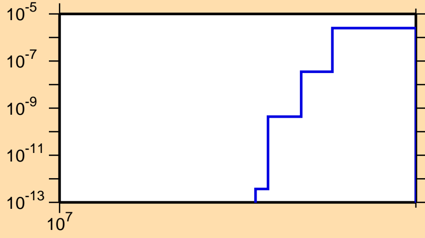
\sigma vs. E for ^{113}\text{Sb}(n,2n\alpha)
