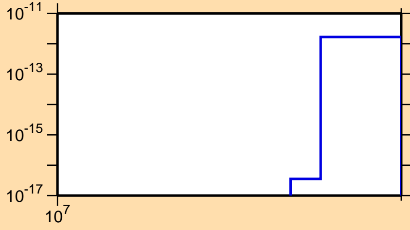
\sigma vs. E for ^{113}\text{Sb} (mt 34)
