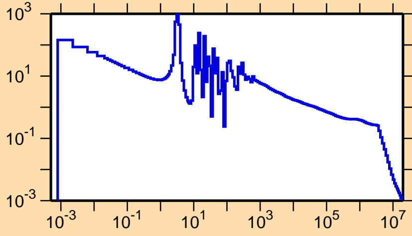
\sigma vs. E for ^{113}\text{Sb}(n,\gamma)
