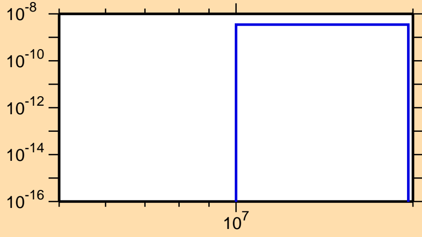
\sigma vs. E for ^{113}\text{Sb}(\text{mt117})
