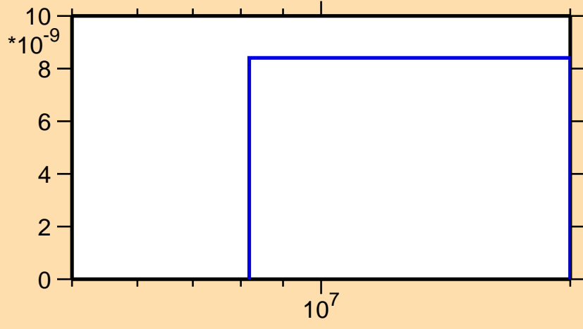
\sigma vs. E for ^{113}\text{Sb}(n,pd)
