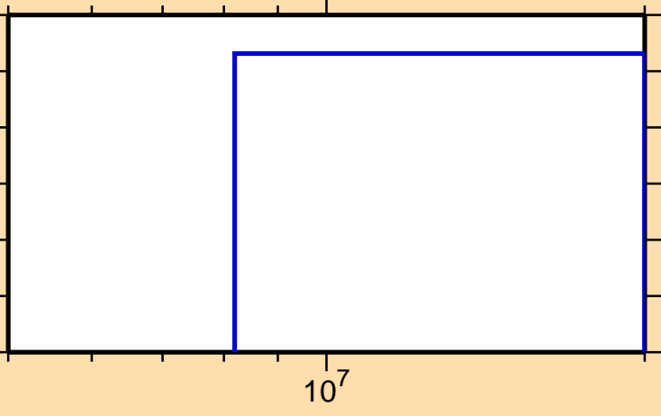
\sigma vs. E for ^{113}\text{Sb}(n,2np)
