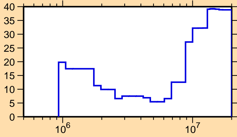
\Delta\sigma/\sigma vs. E for ^{114}\text{Sb}(n,n\text{cont.})
