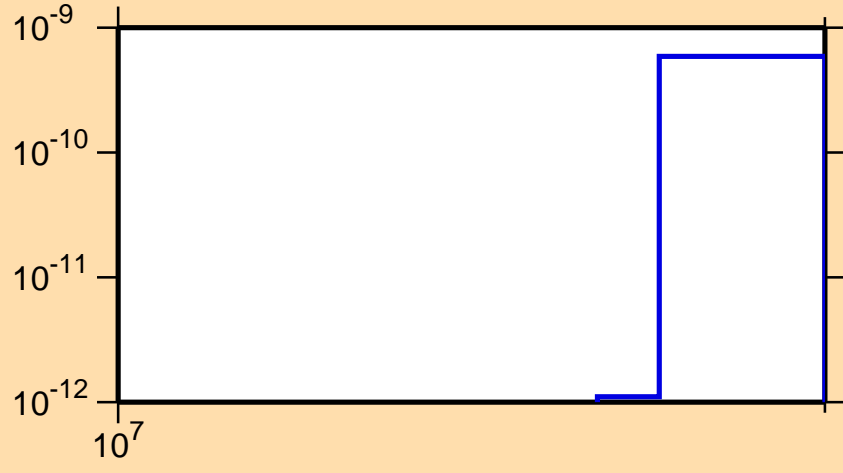
\sigma vs. E for ^{114}\text{Sb} (mt 34)
