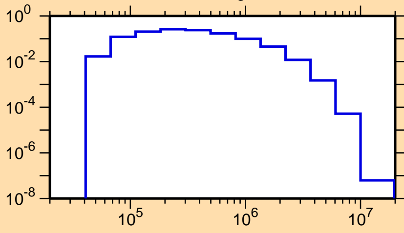
\sigma vs. E for ^{114}\text{Sb}(n,n_3)
