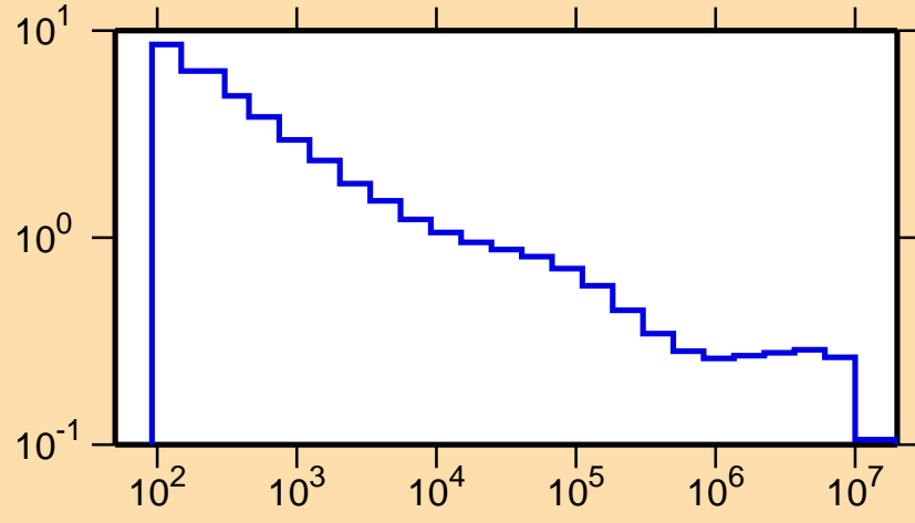
\sigma vs. E for ^{114}\text{Sb}(n,p)
