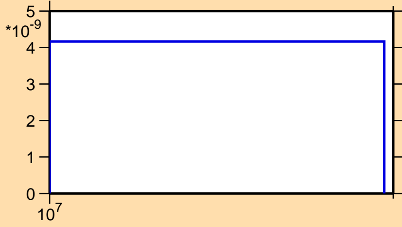
\sigma vs. E for ^{114}\text{Sb} (mt 45)
