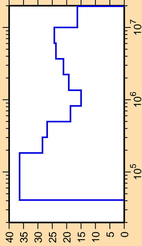
\Delta\sigma/\sigma vs. E for ^{114}\text{Sb}(n,n_3)
