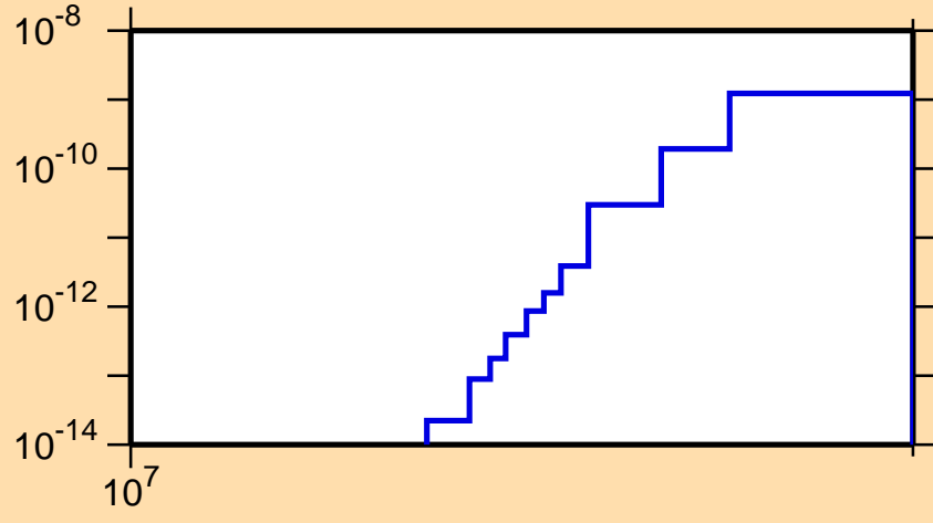
\sigma vs. E for ^{115}\text{Sb}(\text{mt117})
