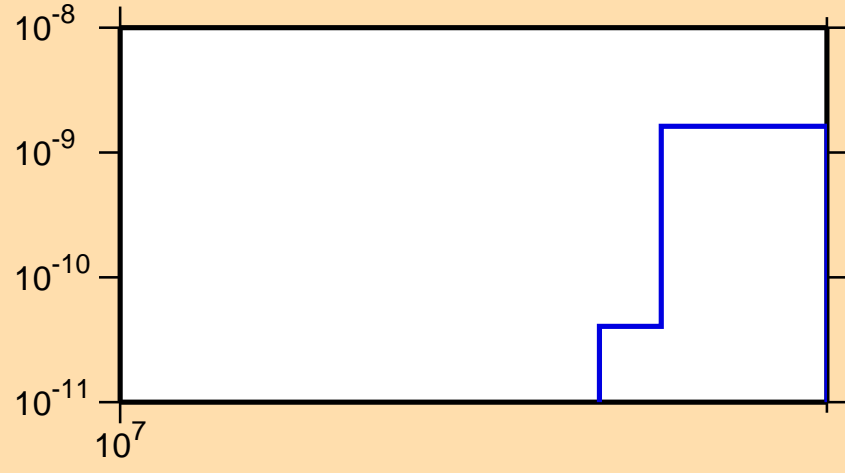
\sigma vs. E for ^{115}\text{Sb}(n,\text{pd})
