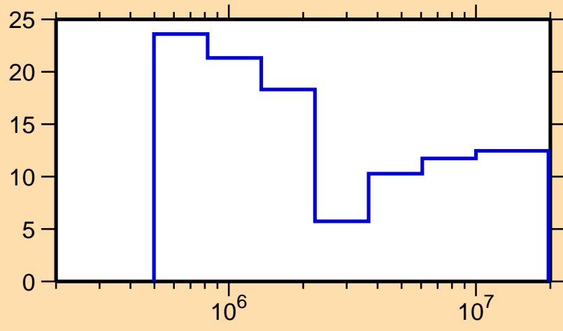
\Delta\sigma/\sigma vs. E for ^{115}\text{Sb}(n,\text{tot.})
