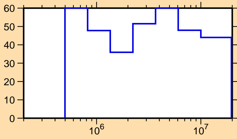
\Delta\sigma/\sigma vs. E for ^{115}\text{Sb}(n,n_1)
