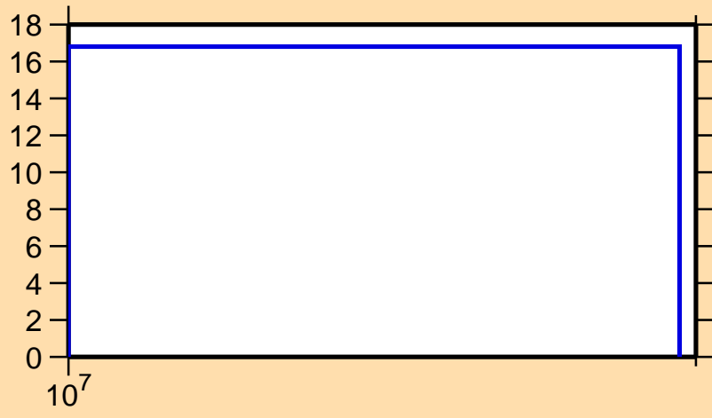
\Delta\sigma/\sigma vs. E for ^{115}\text{Sb}(n,\text{el.})
