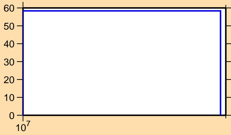
\Delta\sigma/\sigma vs. E for ^{115}\text{Sb}(n,\text{inel.})
