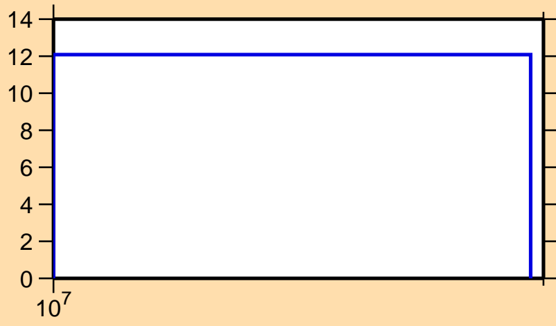
\Delta\sigma/\sigma vs. E for ^{115}\text{Sb}(n,\text{nonel.})
