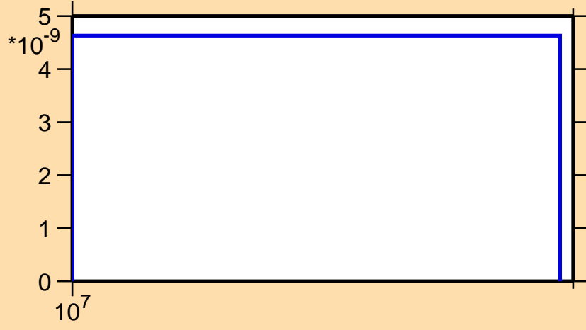
\sigma vs. E for ^{115}\text{Sb}(n,2n\alpha)
