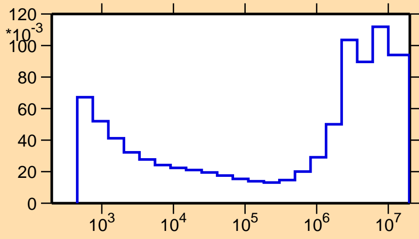
\sigma vs. E for ^{115}\text{Sb}(n,p)
