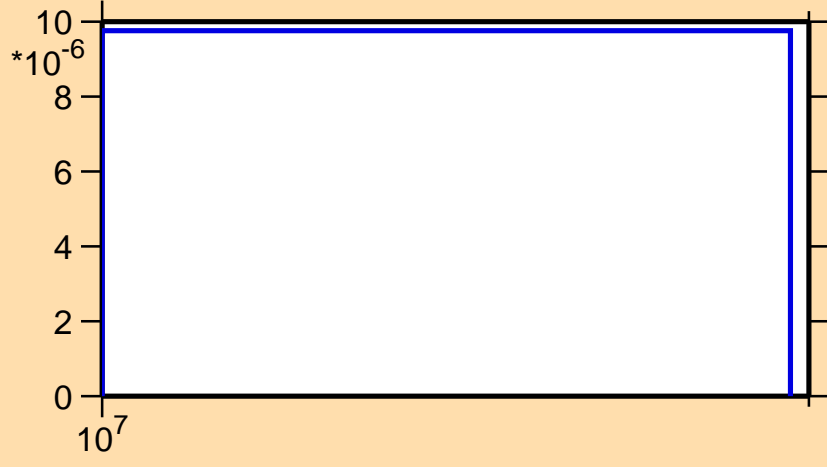
\sigma vs. E for ^{115}\text{Sb}(n,2np)
