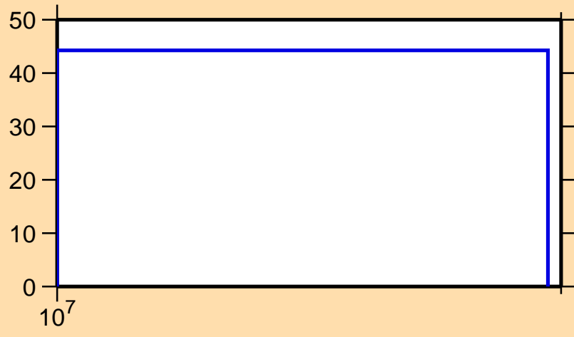
\Delta\sigma/\sigma vs. E for ^{115}\text{Sb}(n,2n)
