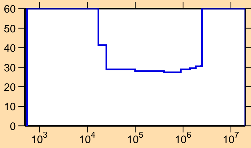
\Delta\sigma/\sigma vs. E for ^{115}\text{Sb}(n,p)
