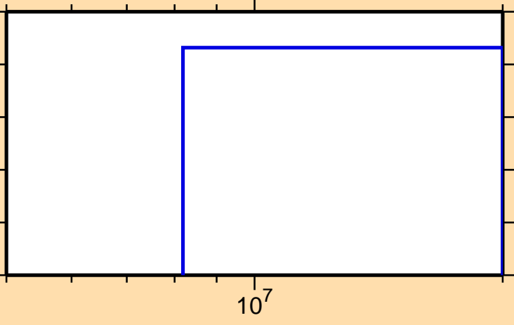
\sigma vs. E for ^{115}\text{Sb}(n,2np)
