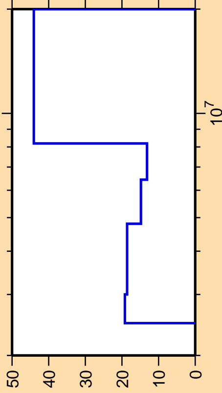
\Delta\sigma/\sigma vs. E for ^{115}\text{Sb}(n,n\text{cont.})
