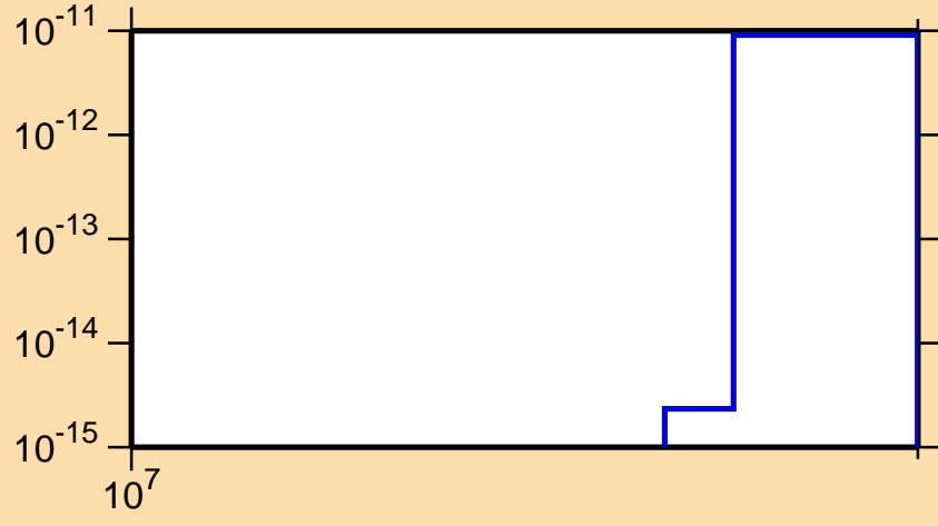
\sigma vs. E for ^{116}\text{Sb}(n,\text{pt})
