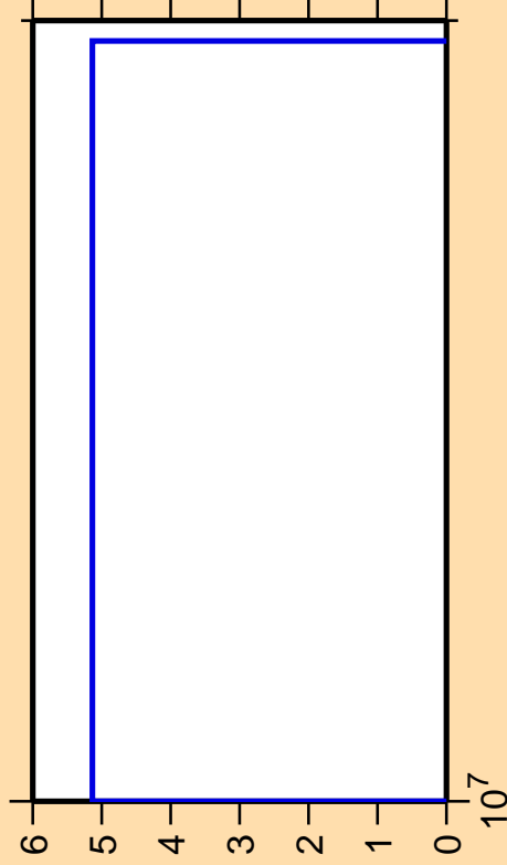
\Delta\sigma/\sigma vs. E for ^{116}\text{Sb} (mt 45)
