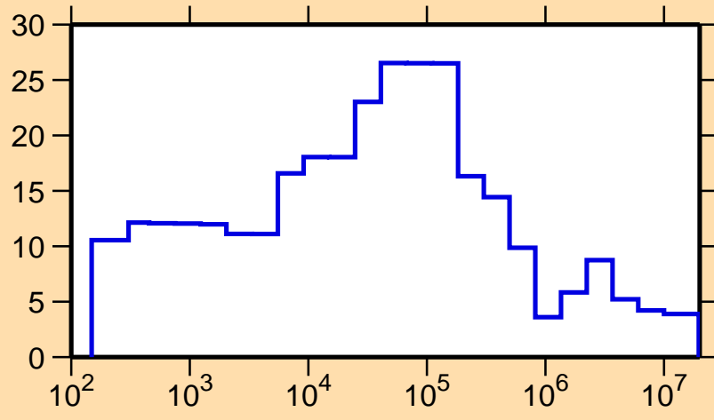
\Delta\sigma/\sigma vs. E for ^{116}\text{Sb}(n,el.)
