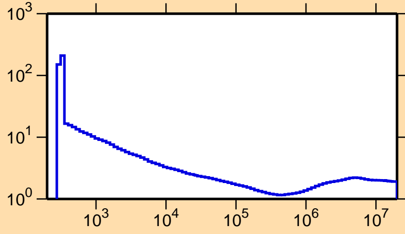
\sigma vs. E for ^{116}\text{Sb}(n,\text{nonel.})
