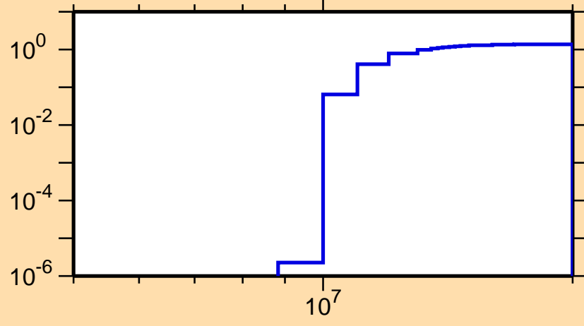
\sigma vs. E for ^{117}\text{Sb}(n,2n)
