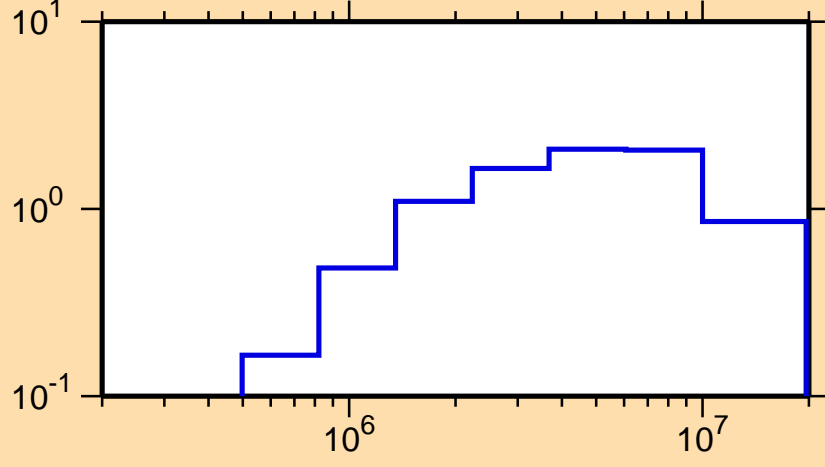
\sigma vs. E for ^{117}\text{Sb}(n,\text{inel.})
