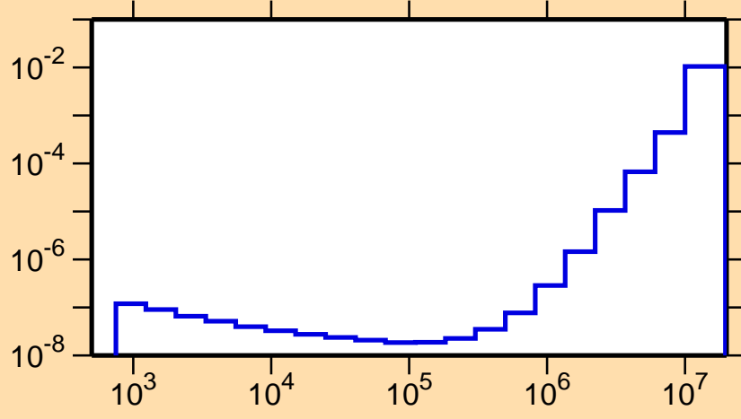
\sigma vs. E for ^{117}\text{Sb}(n,\alpha)
