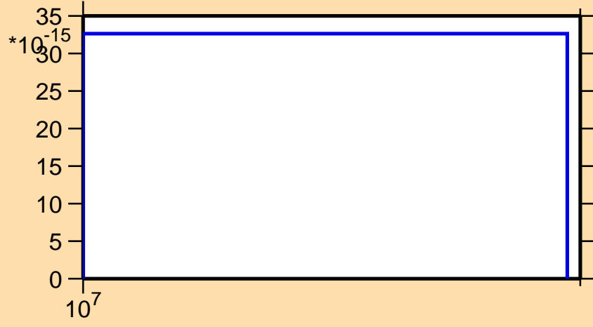
\sigma vs. E for ^{117}\text{Sb}(n,pd)
