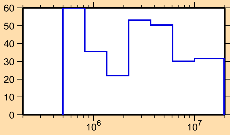
\Delta\sigma/\sigma vs. E for ^{117}\text{Sb}(n,n_1)
