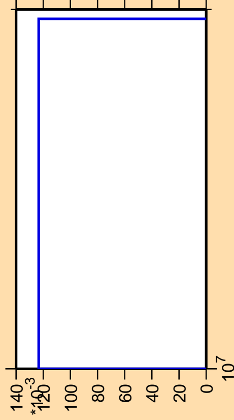
\Delta\sigma/\sigma vs. E for ^{117}\text{Sb}(n,pd)
