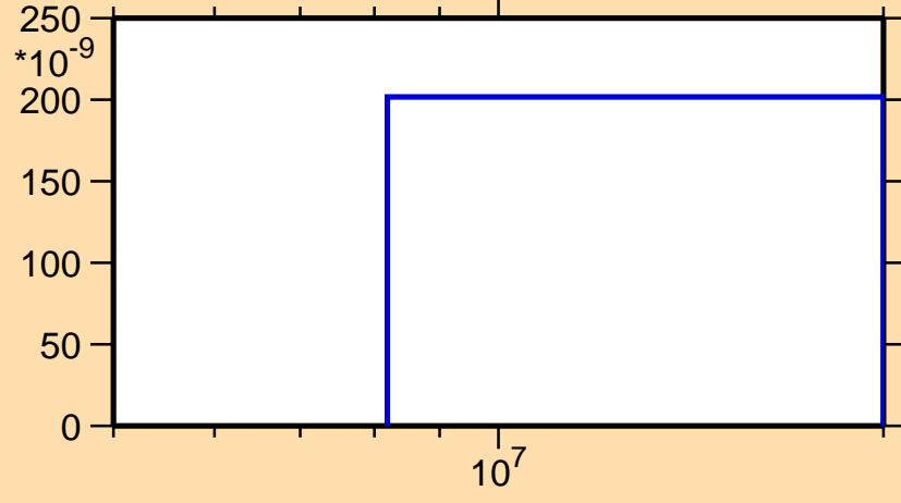
\sigma vs. E for ^{117}\text{Sb}(n,\text{nd})
