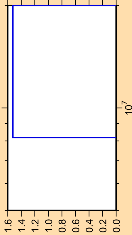
\Delta\sigma/\sigma vs. E for ^{117}\text{Sb}(\text{mt } 45)
