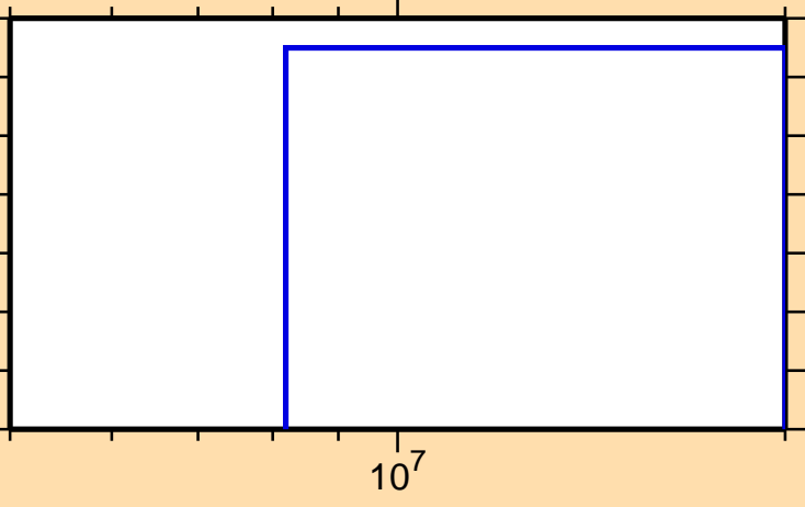
\sigma vs. E for ^{117}\text{Sb}(n,p\alpha)
