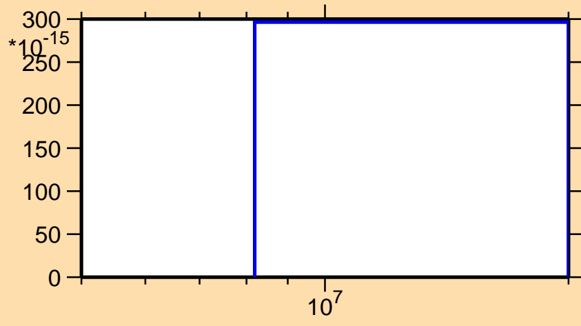
\sigma vs. E for ^{117}\text{Sb}(\text{mt } 45)
