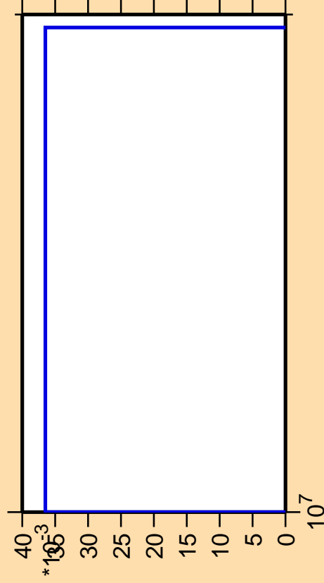
\Delta\sigma/\sigma vs. E for ^{118}\text{Sb}(\text{mt117})
