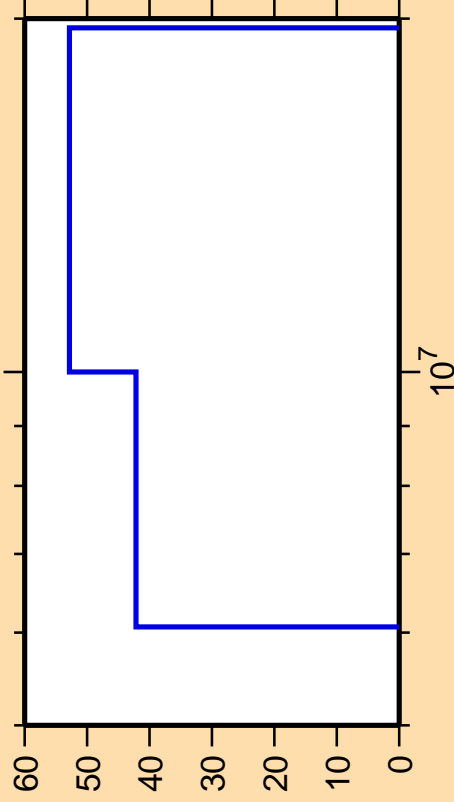
\Delta\sigma/\sigma vs. E for ^{118}\text{Sb}(n,\gamma)
