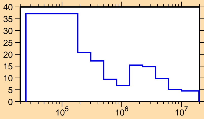
\Delta\sigma/\sigma vs. E for ^{118}\text{Sb}(n,n_1)
