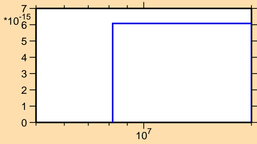
\sigma vs. E for ^{118}\text{Sb}(\text{mt117})
