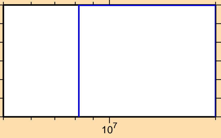
\sigma vs. E for ^{118}\text{Sb}(n,\text{nd})
