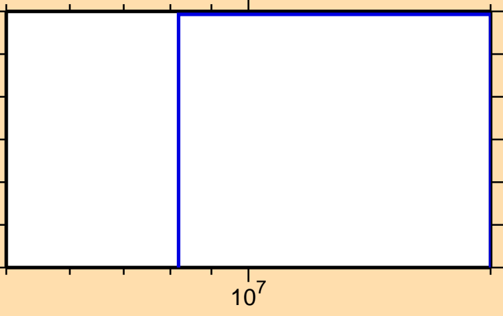
\sigma vs. E for ^{118}\text{Sb}(\text{mt } 45)
