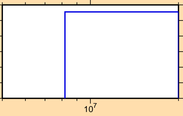
\sigma vs. E for ^{118}\text{Sb}(n,\text{He}3)
