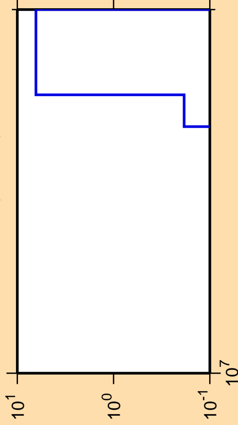
\Delta\sigma/\sigma vs. E for ^{118}\text{Sb}(\text{mt117})
