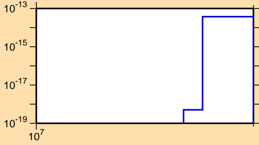
\sigma vs. E for ^{118}\text{Sb}(n,\text{pt})
