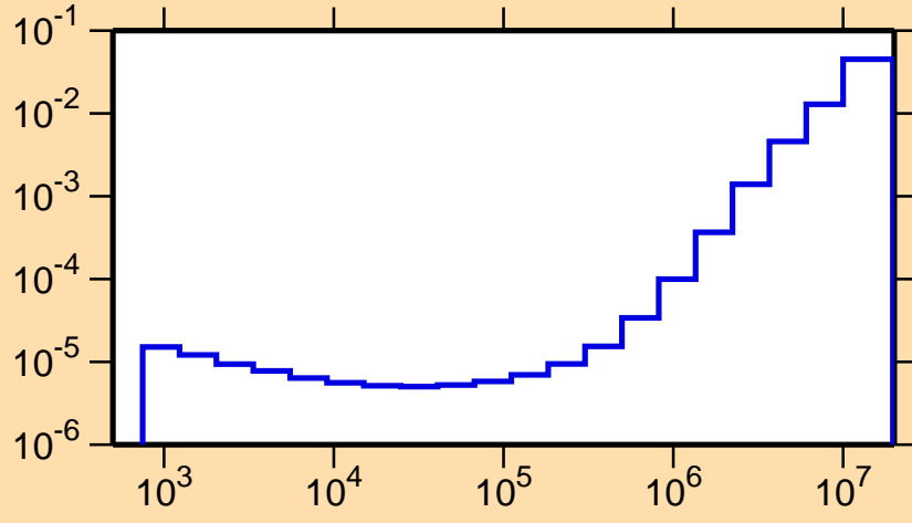
\sigma vs. E for ^{118}\text{Sb}(n,p)
