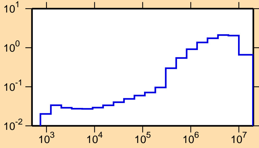
\sigma vs. E for ^{118}\text{Sb}(n,\text{inel.})
