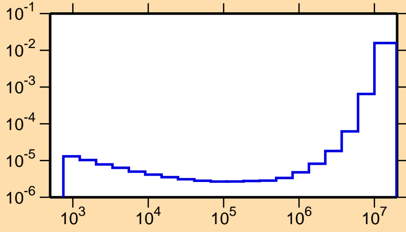
\sigma vs. E for ^{118}\text{Sb}(n,\alpha)
