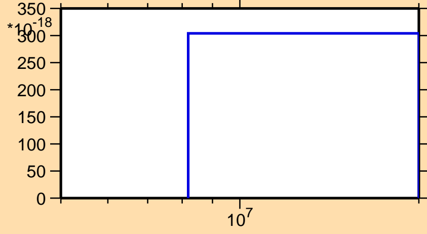
\sigma vs. E for ^{118}\text{Sb}(n,pt)
