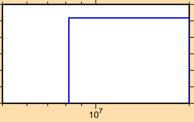
\sigma vs. E for ^{118}\text{Sb}(n,nt)
