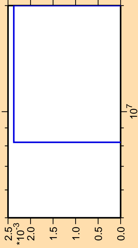
\Delta\sigma/\sigma vs. E for ^{118}\text{Sb}(n,pt)
