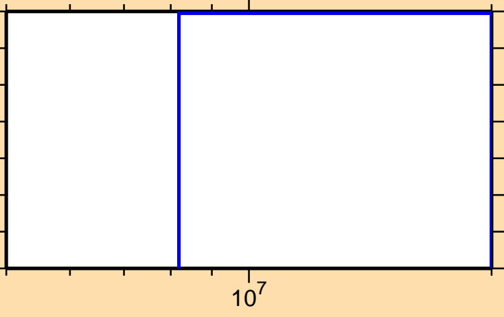
\sigma vs. E for ^{118}\text{Sb}(\text{mt } 34)
