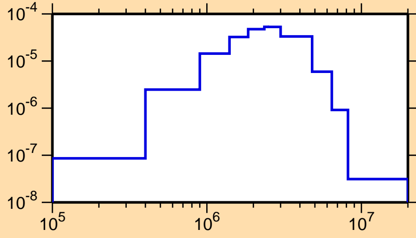
\sigma vs. E for ^{118}\text{Sb}(n,n_1)
