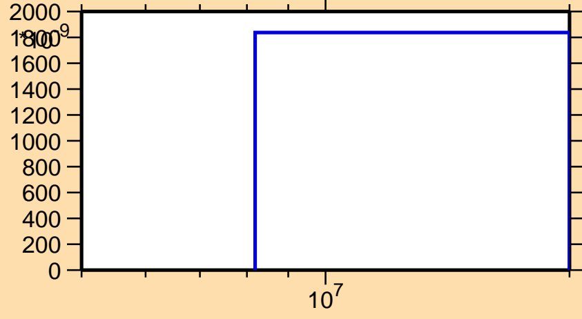
\sigma vs. E for ^{118}\text{Sb}(n,nd)
