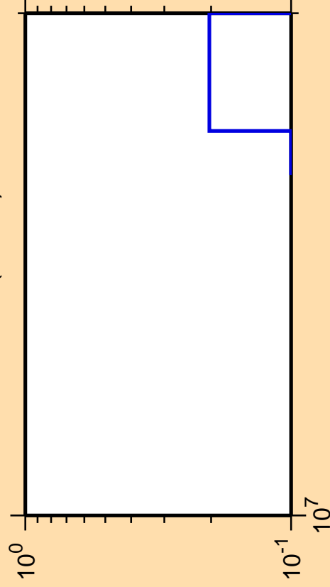
\Delta\sigma/\sigma vs. E for ^{119}\text{Sb} (mt 45)
