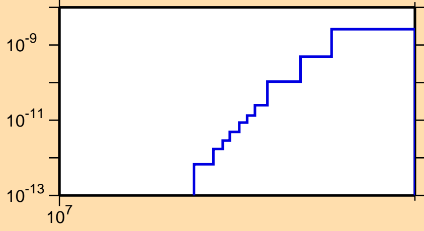
\sigma vs. E for ^{119}\text{Sb}(n,p\alpha)
