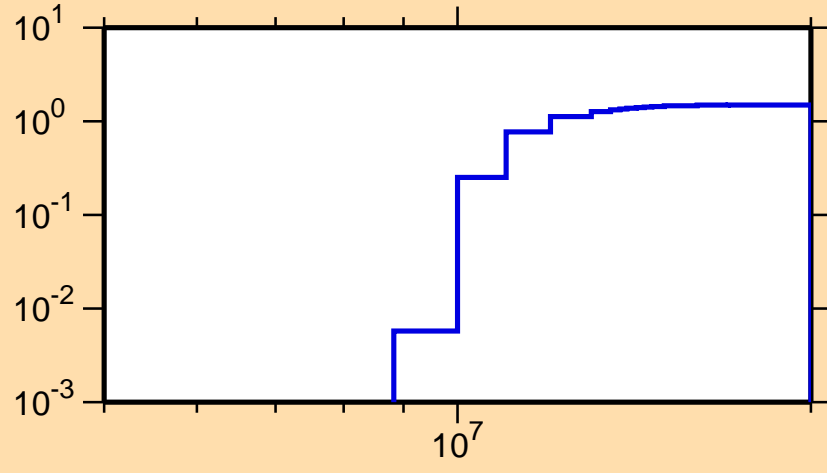
\sigma vs. E for ^{119}\text{Sb}(n,2n)
