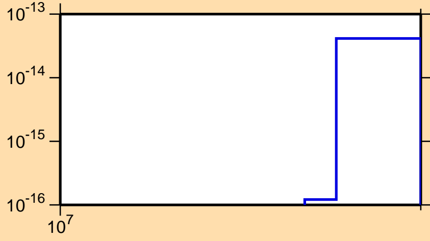
\sigma vs. E for ^{119}\text{Sb} (mt 45)
