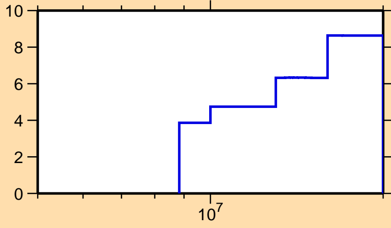
\Delta\sigma/\sigma vs. E for ^{119}\text{Sb}(n,\text{tot.})
