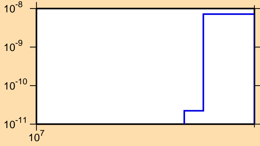
\sigma vs. E for ^{119}\text{Sb}(n,2n\alpha)
