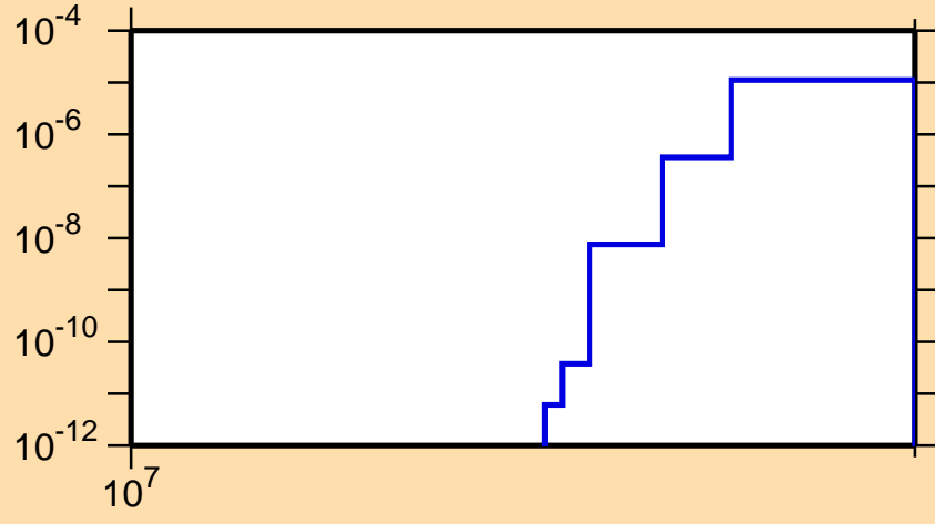
\sigma vs. E for ^{119}\text{Sb}(n,nd)
