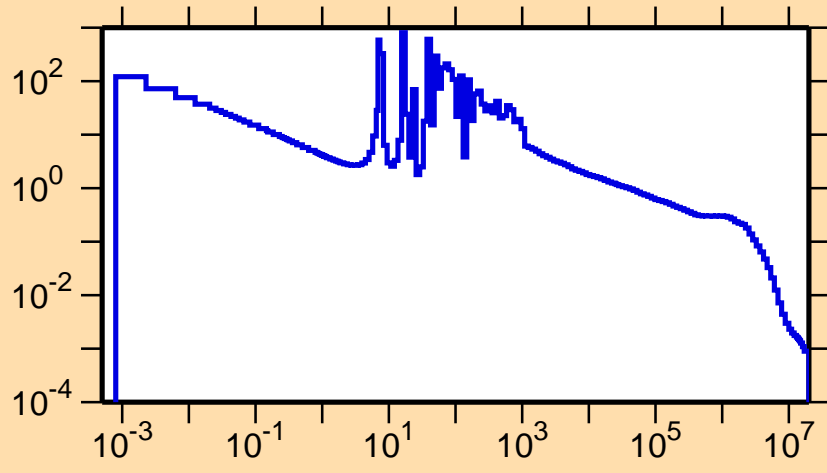
\sigma vs. E for ^{119}\text{Sb}(n,\gamma)
