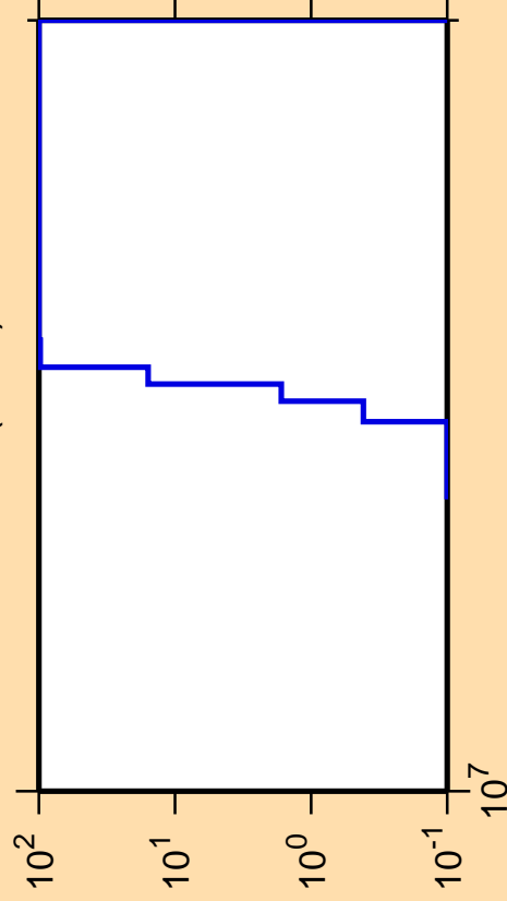
\Delta\sigma/\sigma vs. E for ^{119}\text{Sb}(n,nd)
