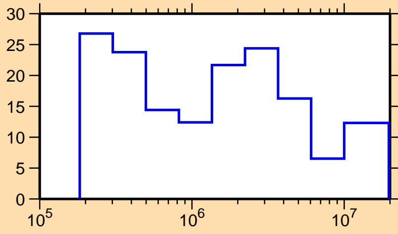
\Delta\sigma/\sigma vs. E for ^{119}\text{Sb}(n,\text{el.})
