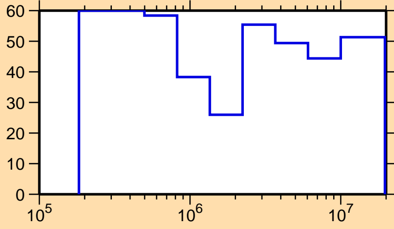
\Delta\sigma/\sigma vs. E for ^{119}\text{Sb}(n,n_1)
