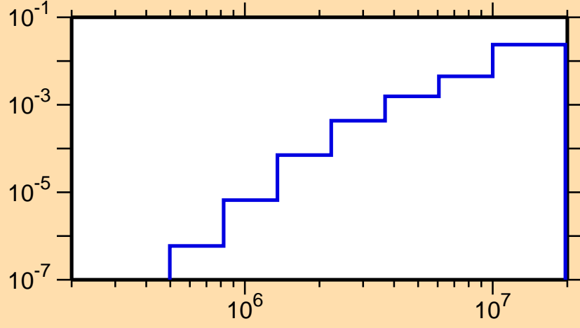
\sigma vs. E for ^{119}\text{Sb}(n,p)
