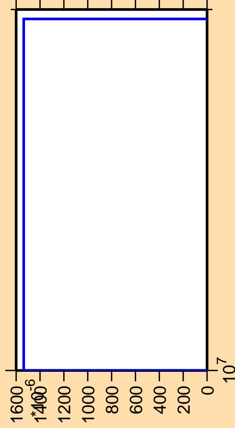
\Delta\sigma/\sigma vs. E for ^{119}\text{Sb} (mt 45)
