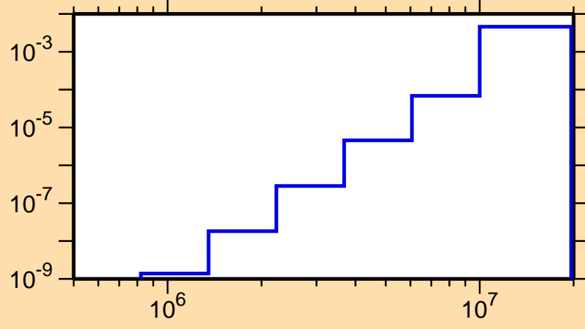
\sigma vs. E for ^{119}\text{Sb}(n,\alpha)
