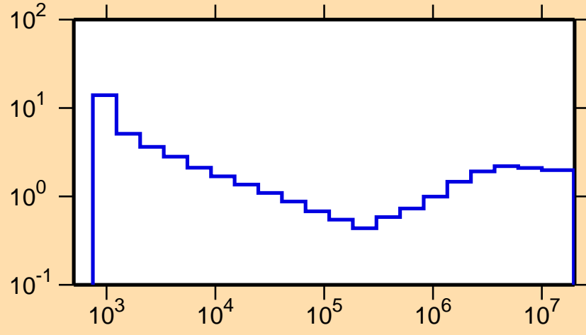
\sigma vs. E for ^{119}\text{Sb}(n,\text{nonel.})
