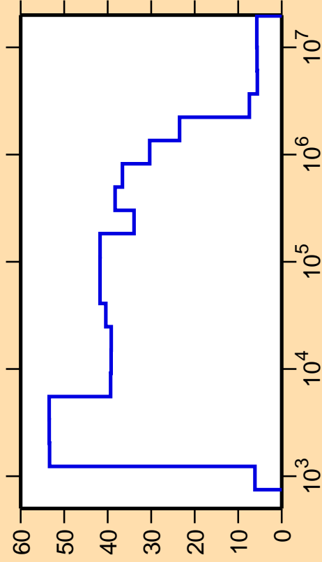
\Delta\sigma/\sigma vs. E for ^{119}\text{Sb}(n,\text{nonel.})
