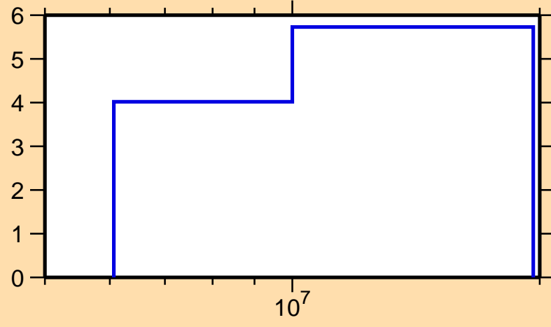
\Delta\sigma/\sigma vs. E for ^{119}\text{Sb}(n,\text{tot.})
