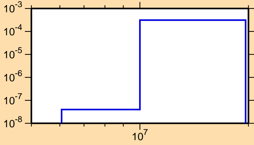
\sigma vs. E for ^{119}\text{Sb}(n,n\alpha)
