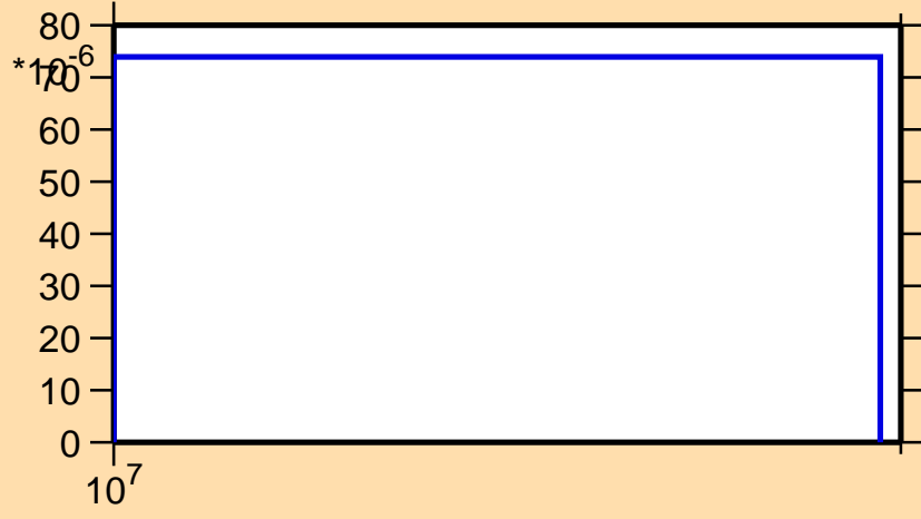
\sigma vs. E for ^{119}\text{Sb}(n,3n)
