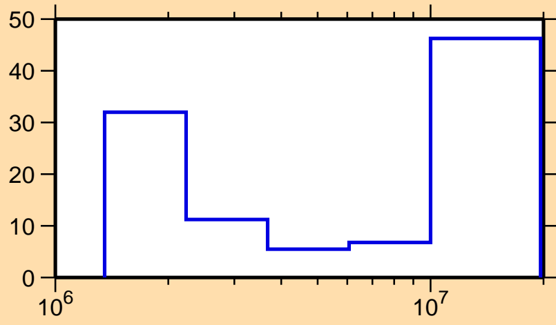
\Delta\sigma/\sigma vs. E for ^{119}\text{Sb}(n,\text{inel.})
