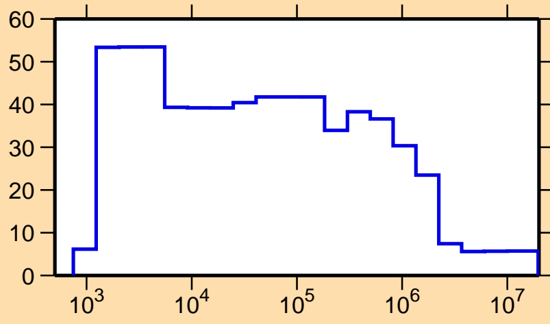
\Delta\sigma/\sigma vs. E for ^{119}\text{Sb}(n,\text{nonel.})
