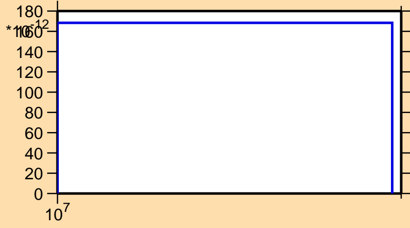
\sigma vs. E for ^{119}\text{Sb}(n,\text{He3})
