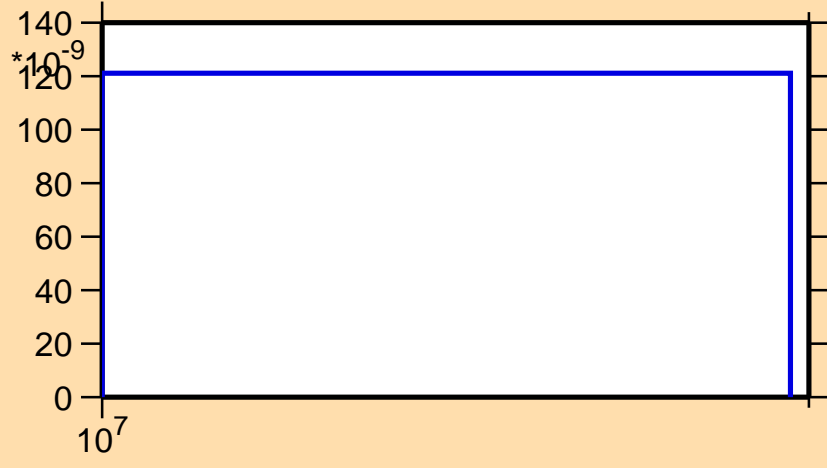
\sigma vs. E for ^{119}\text{Sb}(n,\text{nd})
