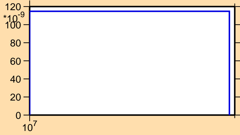
\sigma vs. E for ^{119}\text{Sb}(n,2np)
