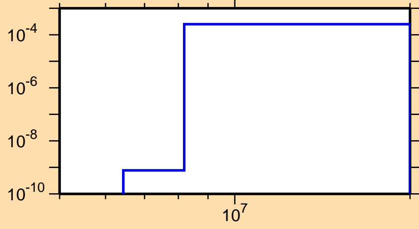
\sigma vs. E for ^{119}\text{Sb}(n,n\alpha)
