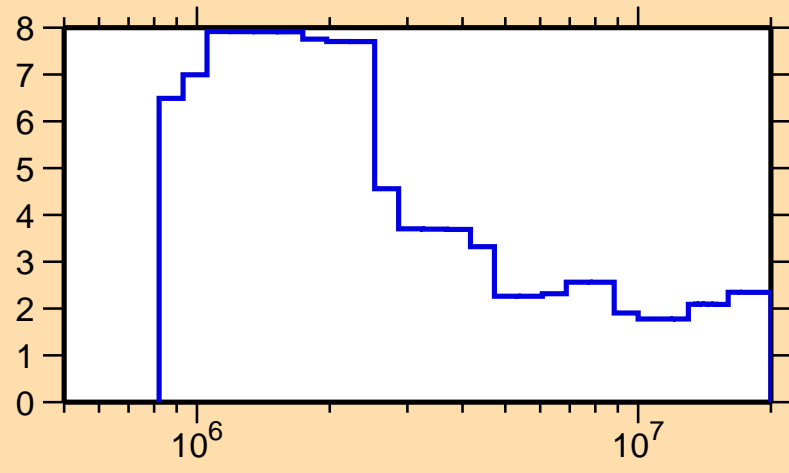
\Delta\sigma/\sigma vs. E for ^{120}\text{Sb}(n,n\text{onel.})
