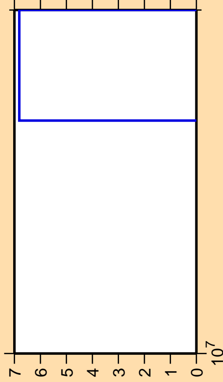
\Delta\sigma/\sigma vs. E for ^{120}\text{Sb}(n,3n)
