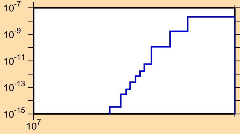
\sigma vs. E for ^{120}\text{Sb}(n,\text{He3})
