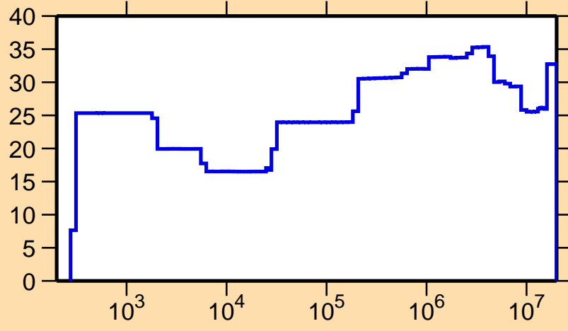
\Delta\sigma/\sigma vs. E for ^{120}\text{Sb}(n,\gamma)
