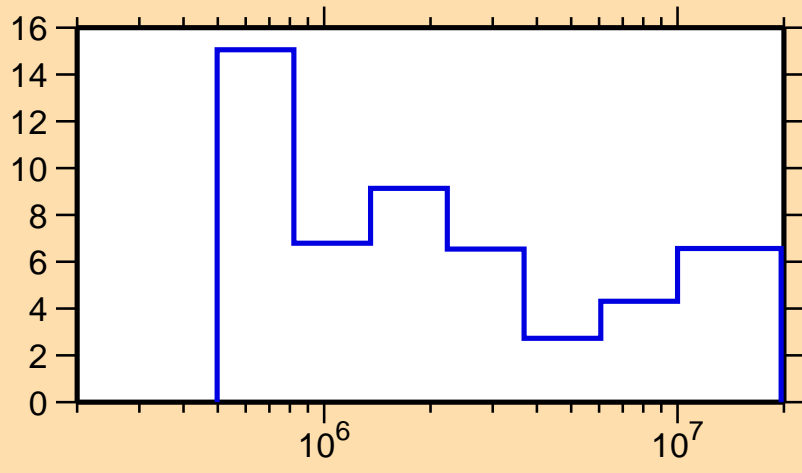
\Delta\sigma/\sigma vs. E for ^{120}\text{Sb}(n,\text{tot.})
