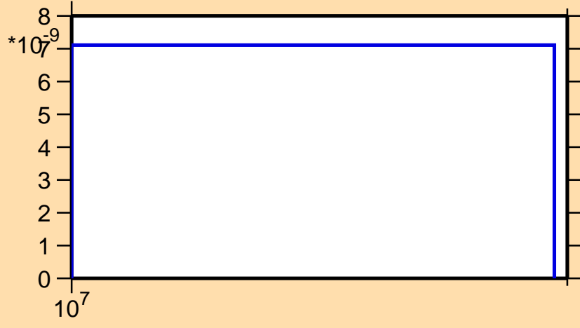
\sigma vs. E for ^{120}\text{Sb}(n,2n\alpha)
