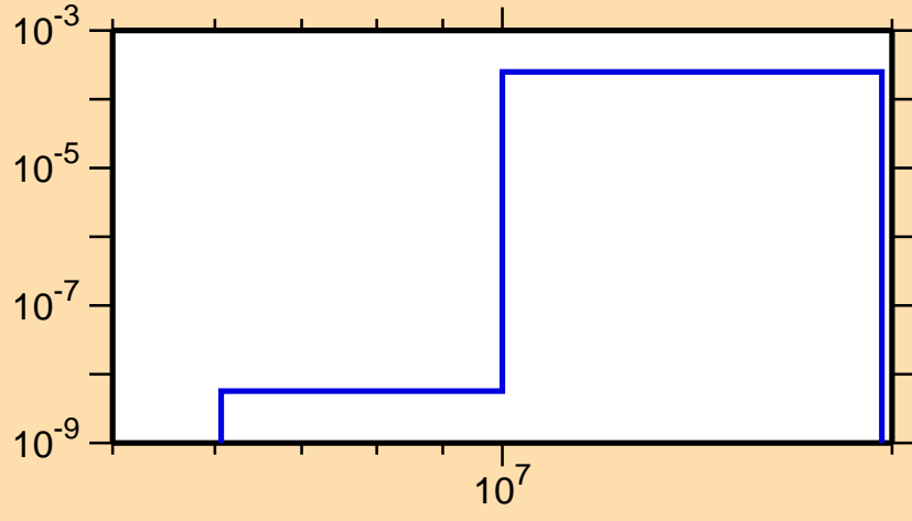
\sigma vs. E for ^{120}\text{Sb}(n,n\alpha)
