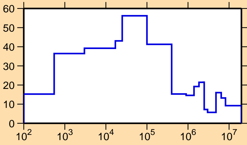
\Delta\sigma/\sigma vs. E for ^{120}\text{Sb}(n,el.)
