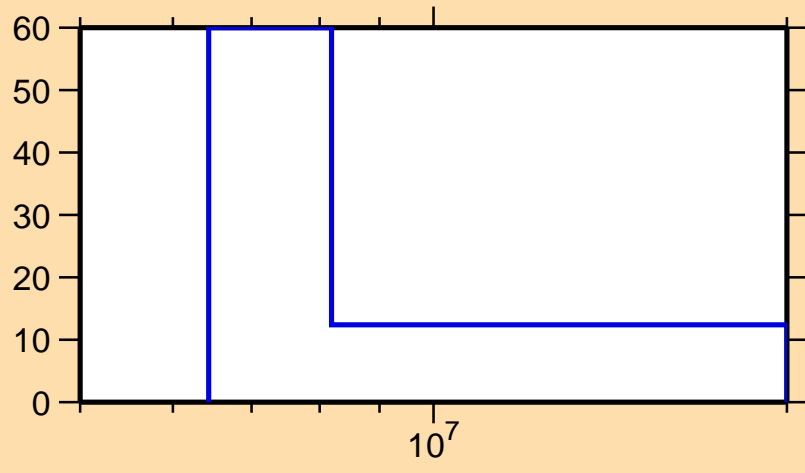
\Delta\sigma/\sigma vs. E for ^{120}\text{Sb}(n,2n)
