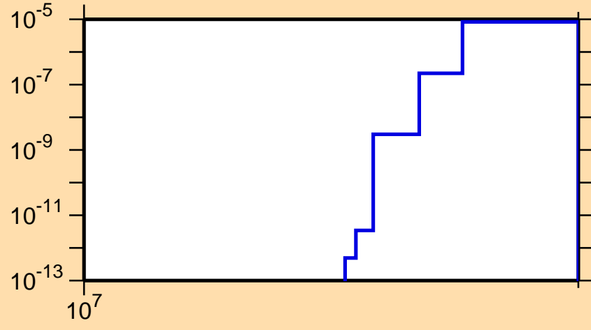
\sigma vs. E for ^{121}\text{Sb}(n,\text{nd})
