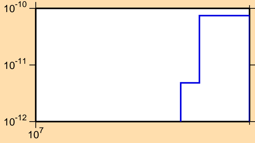
\sigma vs. E for ^{121}\text{Sb}(n,p\alpha)
