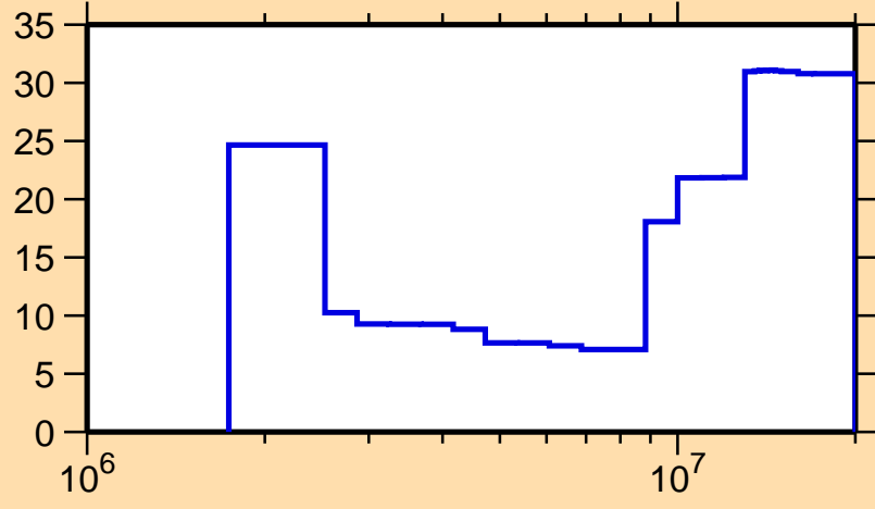
\Delta\sigma/\sigma vs. E for ^{121}\text{Sb}(n,n\text{cont.})
