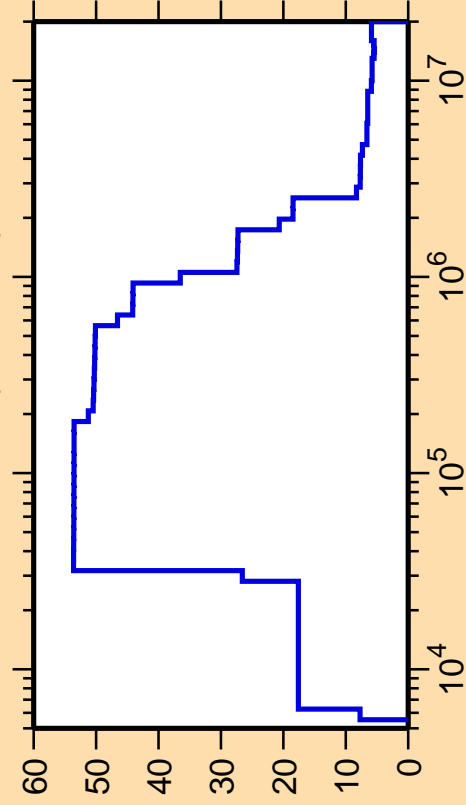
\Delta\sigma/\sigma vs. E for ^{121}\text{Sb}(n,\text{nonel.})
