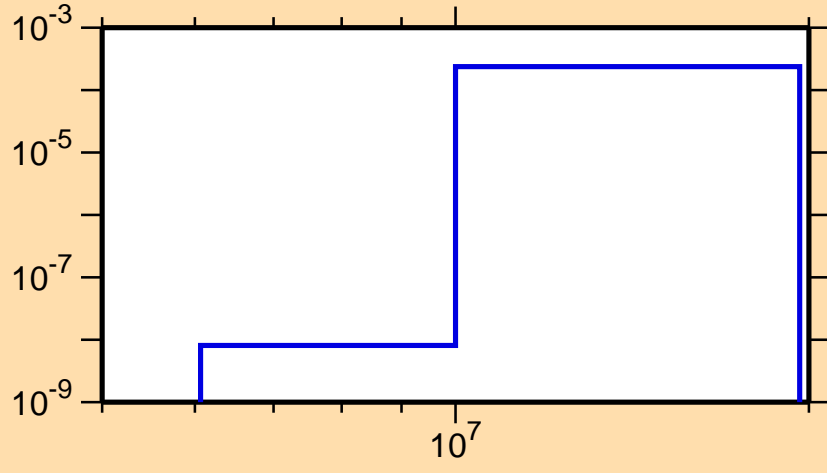
\sigma vs. E for ^{121}\text{Sb}(n,n\alpha)
