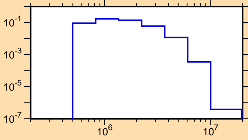
\sigma vs. E for ^{121}\text{Sb}(n,n_2)
