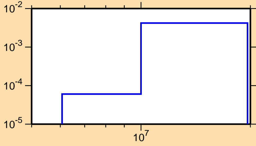
\sigma vs. E for ^{121}\text{Sb}(n,np)
