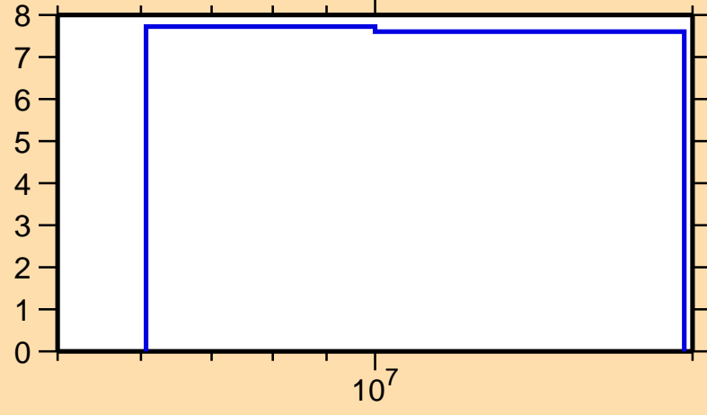
\Delta\sigma/\sigma vs. E for ^{121}\text{Sb}(n,\text{el.})
