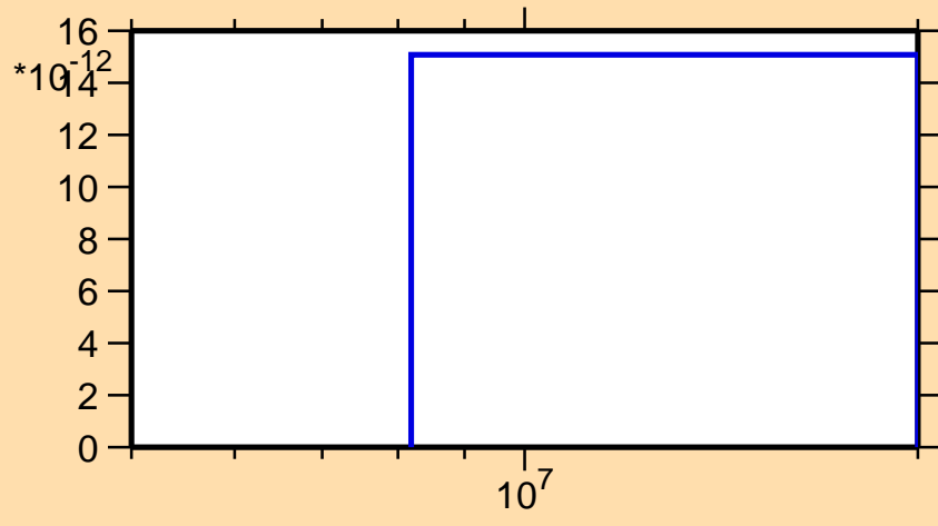
\sigma vs. E for ^{121}\text{Sb}(n,2n\alpha)
