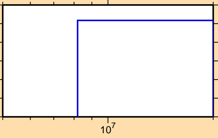
\sigma vs. E for ^{121}\text{Sb}(n,nt)
