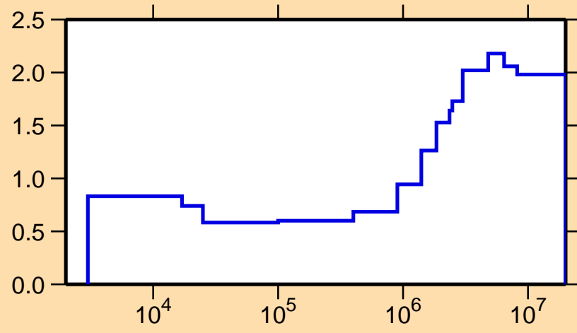
\sigma vs. E for ^{121}\text{Sb}(n,\text{nonel.})
