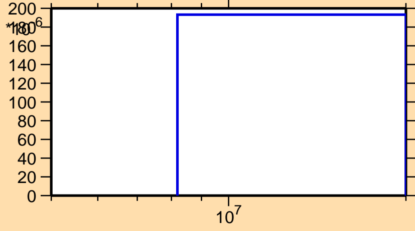
\sigma vs. E for ^{121}\text{Sb}(n,t)
