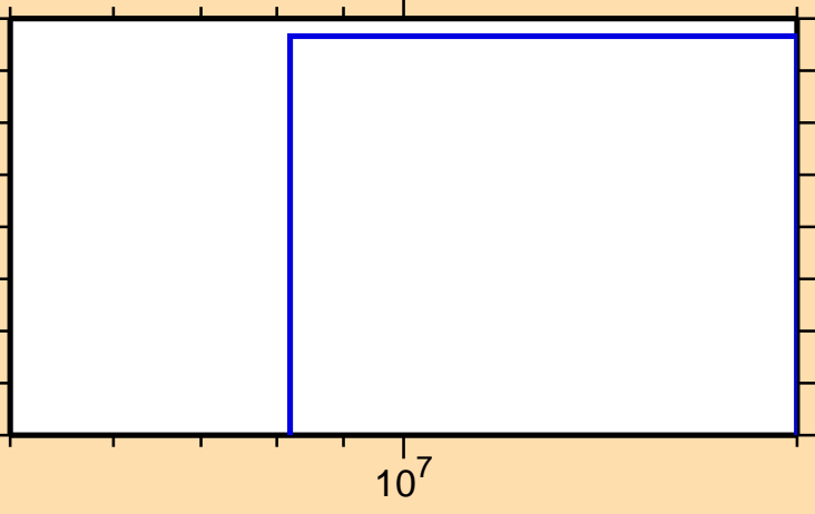
\sigma vs. E for ^{121}\text{Sb}(n,\text{nd})
