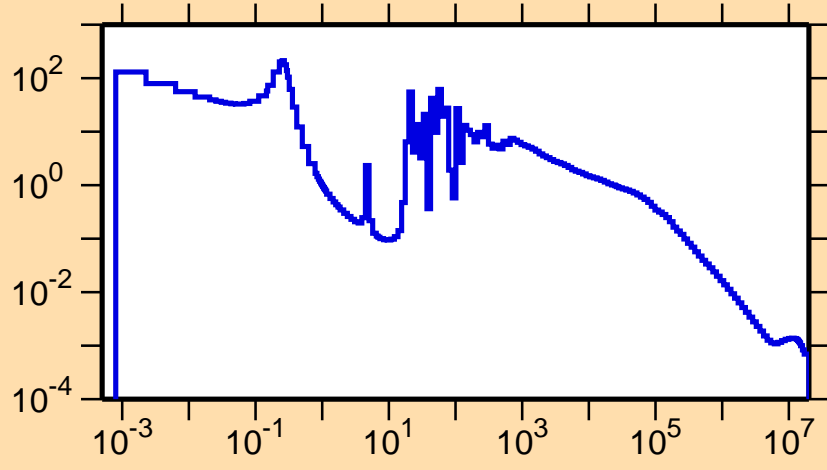
\sigma vs. E for ^{122}\text{Sb}(n,\gamma)
