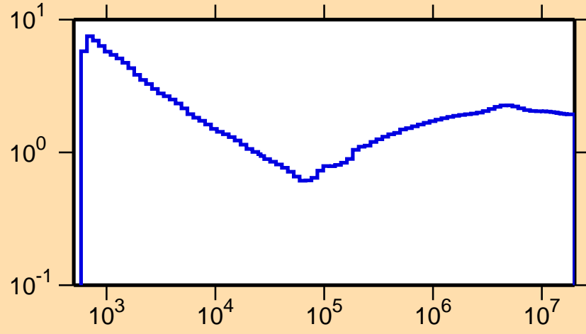
\sigma vs. E for ^{122}\text{Sb}(n,\text{nonel.})
