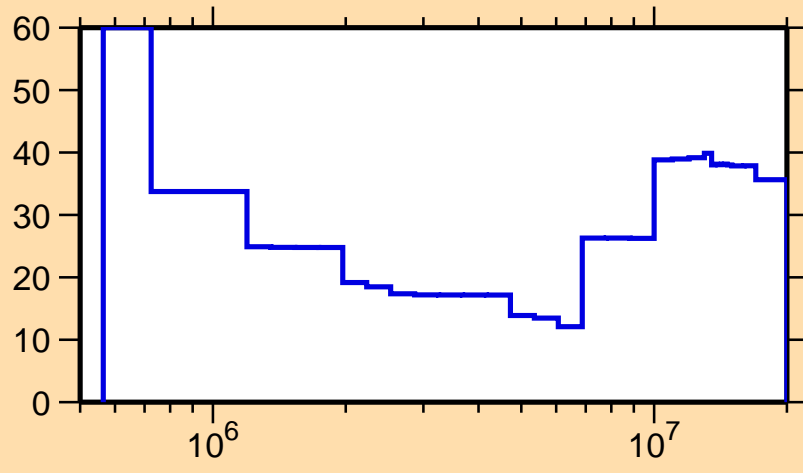
\Delta\sigma/\sigma vs. E for ^{122}\text{Sb}(n,n\text{cont.})
