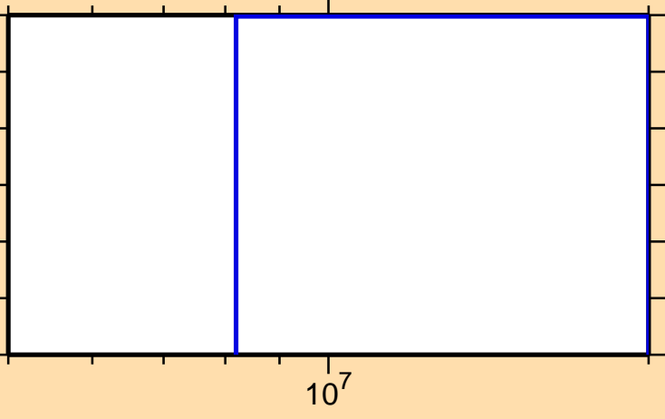
\sigma vs. E for ^{122}\text{Sb}(n,nt)
