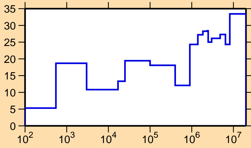
\Delta\sigma/\sigma vs. E for ^{122}\text{Sb}(n,\gamma)
