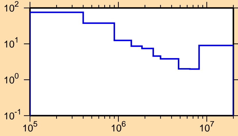
\Delta\sigma/\sigma vs. E for ^{122}\text{Sb}(n,n\text{cont.})
