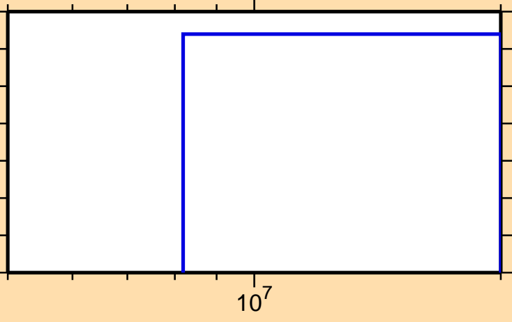
\sigma vs. E for ^{122}\text{Sb}(n,p\alpha)
