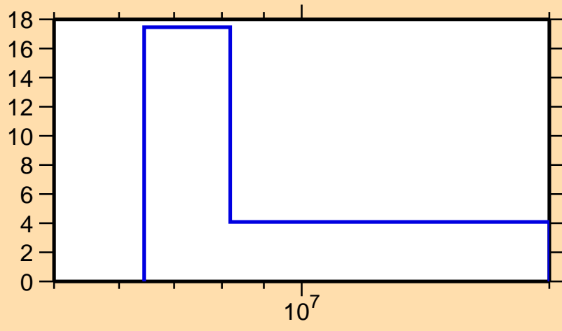
\Delta\sigma/\sigma vs. E for ^{122}\text{Sb}(n,2n)
